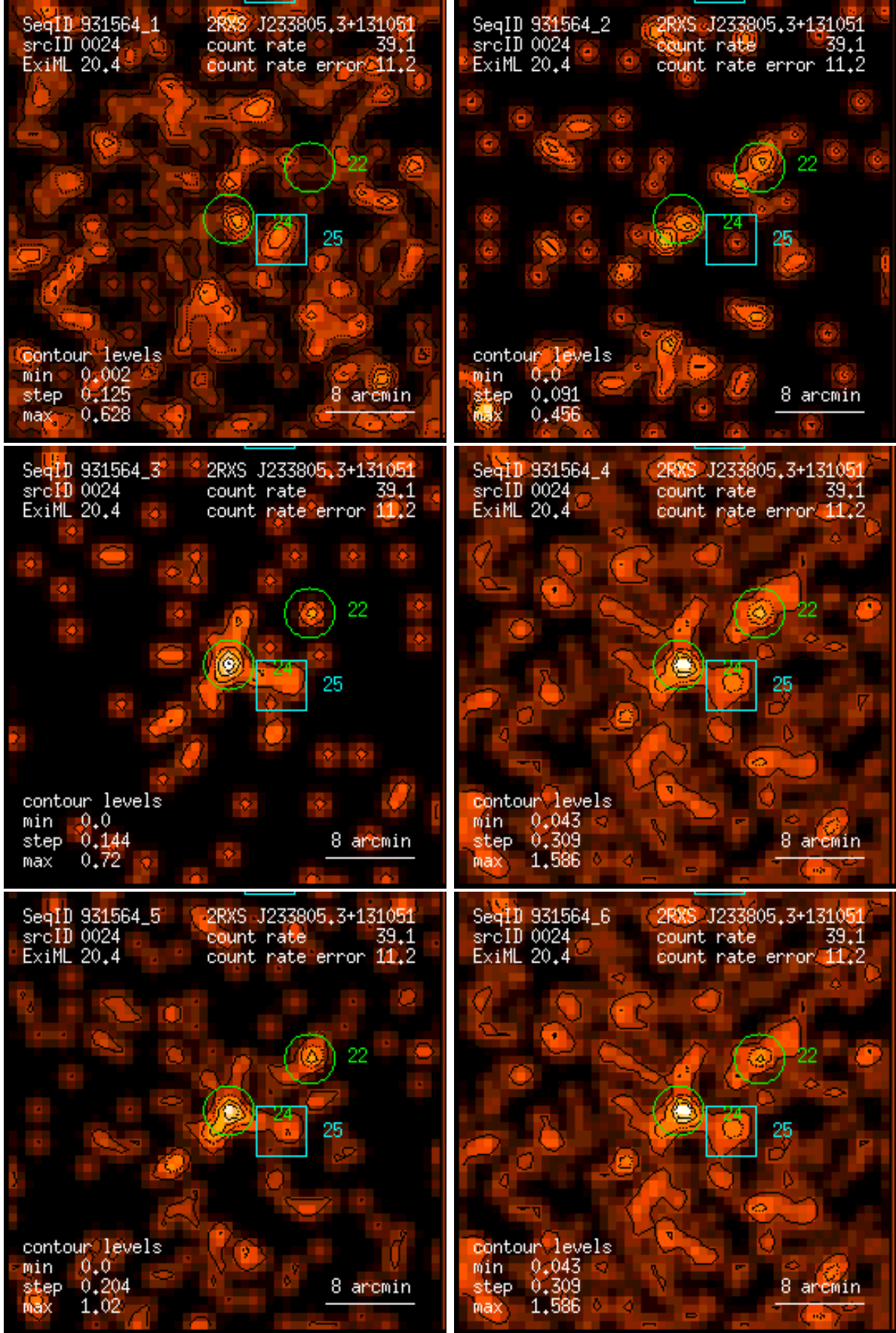
Figure 24: RASS 931564: detection 0024: band rate images, Gaussian filter: (1) PSPC channels 11 – 41, (2) 52 – 90, (3) 91 – 201, (4) 11 – 235, (5) 52 – 201, (6) 11 – 201. Broad band rates in counts/ks. Band rate contour levels in counts/ks/arcmin 2 .
