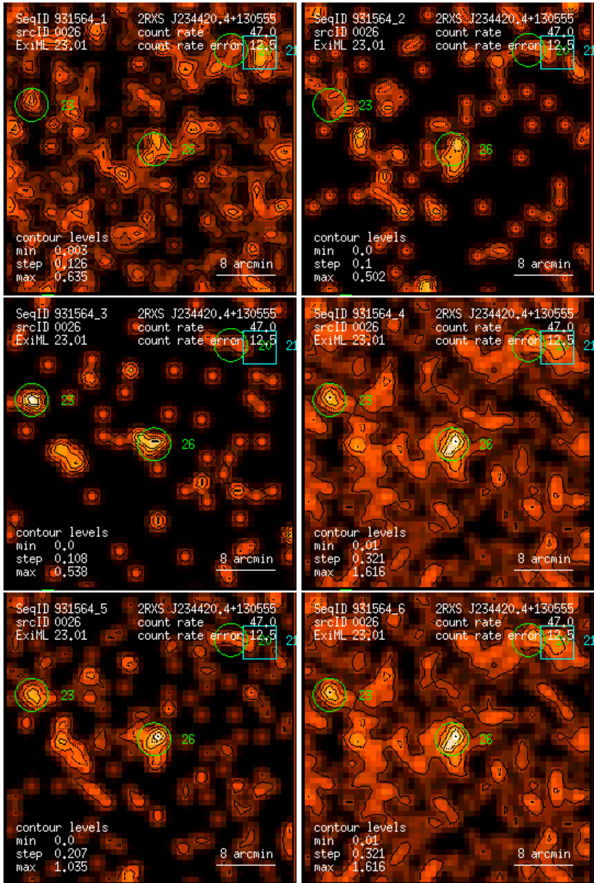
Figure 26: RASS 931564: detection 0026: band rate images, Gaussian filter: (1) PSPC channels 11 – 41, (2) 52 – 90, (3) 91 – 201, (4) 11 – 235, (5) 52 – 201, (6) 11 – 201. Broad band rates in counts/ks. Band rate contour levels in counts/ks/arcmin 2 .
