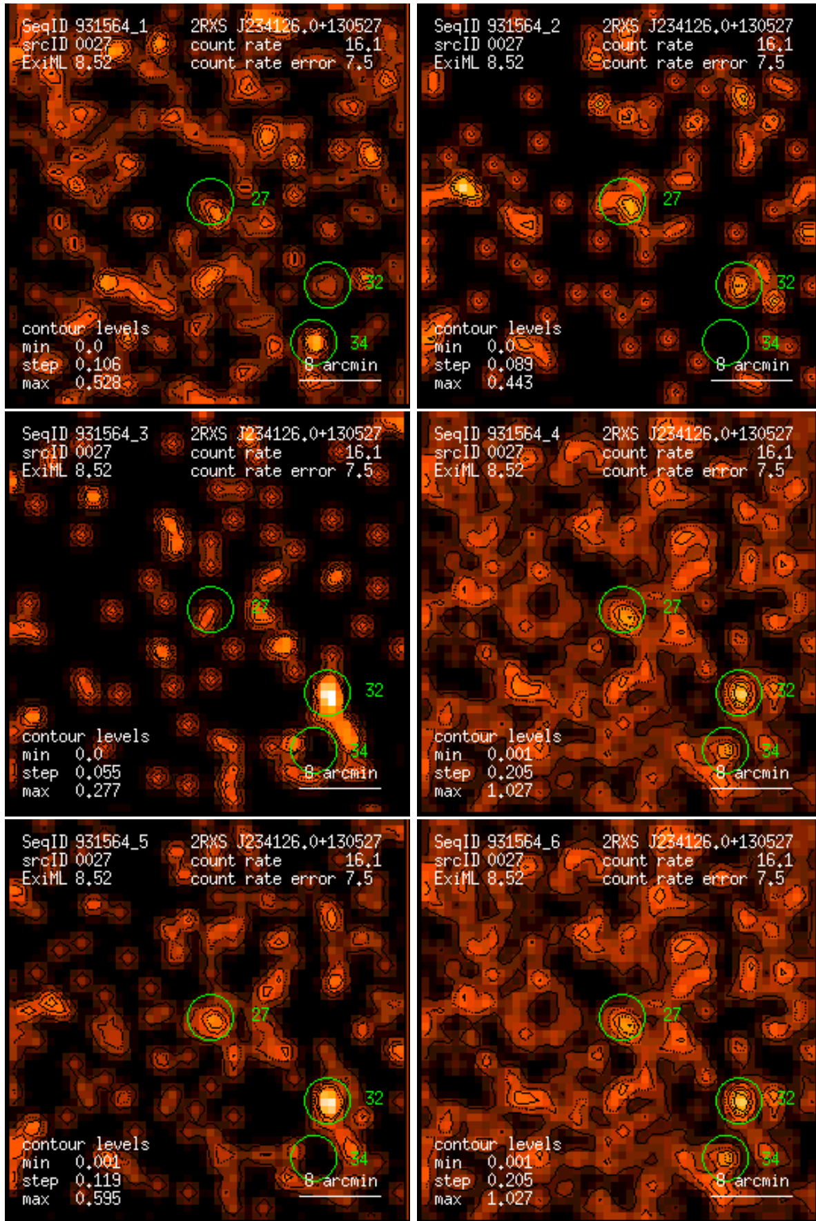
Figure 27: RASS 931564: detection 0027: band rate images, Gaussian filter: (1) PSPC channels 11 – 41, (2) 52 – 90, (3) 91 – 201, (4) 11 – 235, (5) 52 – 201, (6) 11 – 201. Broad band rates in counts/ks. Band rate contour levels in counts/ks/arcmin 2 .
