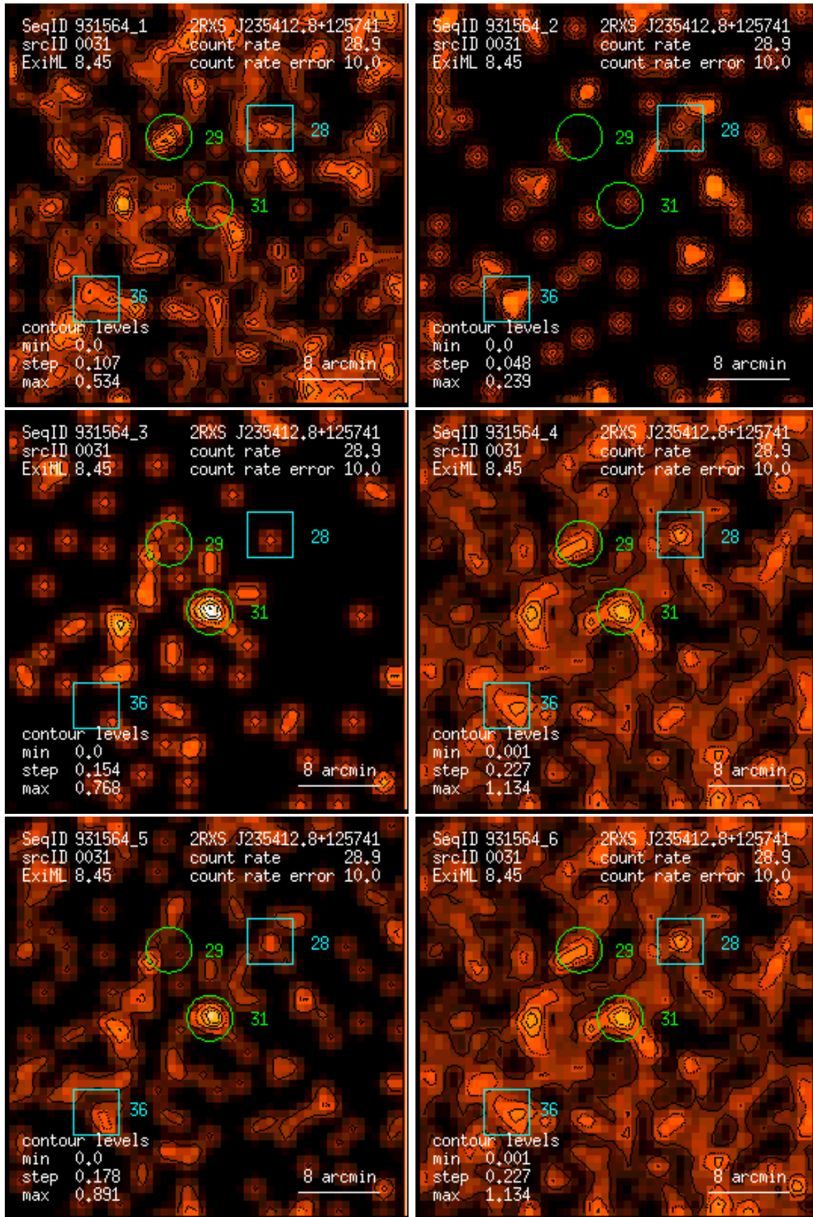
Figure 31: RASS 931564: detection 0031: band rate images, Gaussian filter: (1) PSPC channels 11 – 41, (2) 52 – 90, (3) 91 – 201, (4) 11 – 235, (5) 52 – 201, (6) 11 – 201. Broad band rates in counts/ks. Band rate contour levels in counts/ks/arcmin 2 .
