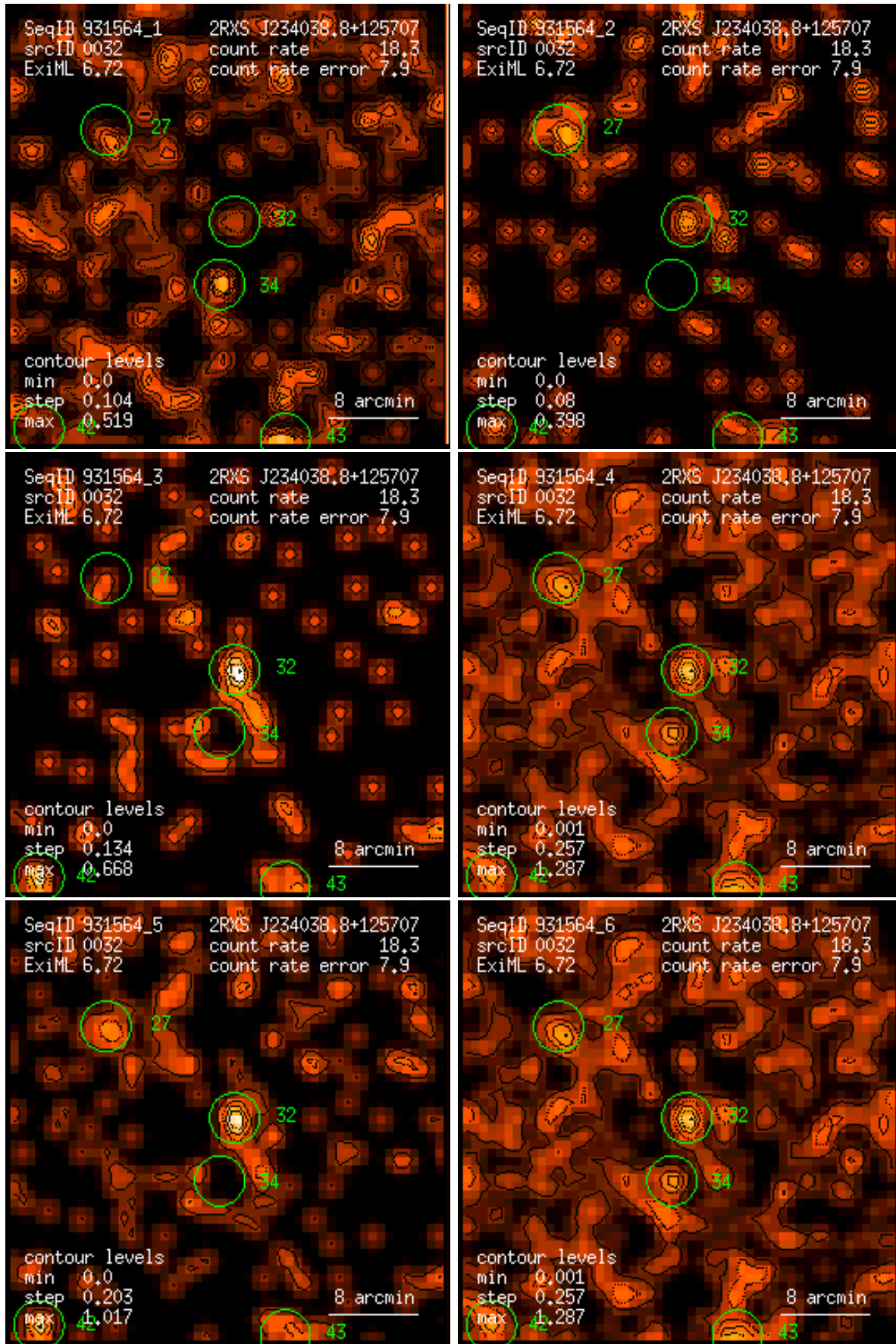
Figure 32: RASS 931564: detection 0032: band rate images, Gaussian filter: (1) PSPC channels 11 – 41, (2) 52 – 90, (3) 91 – 201, (4) 11 – 235, (5) 52 – 201, (6) 11 – 201. Broad band rates in counts/ks. Band rate contour levels in counts/ks/arcmin 2 .
