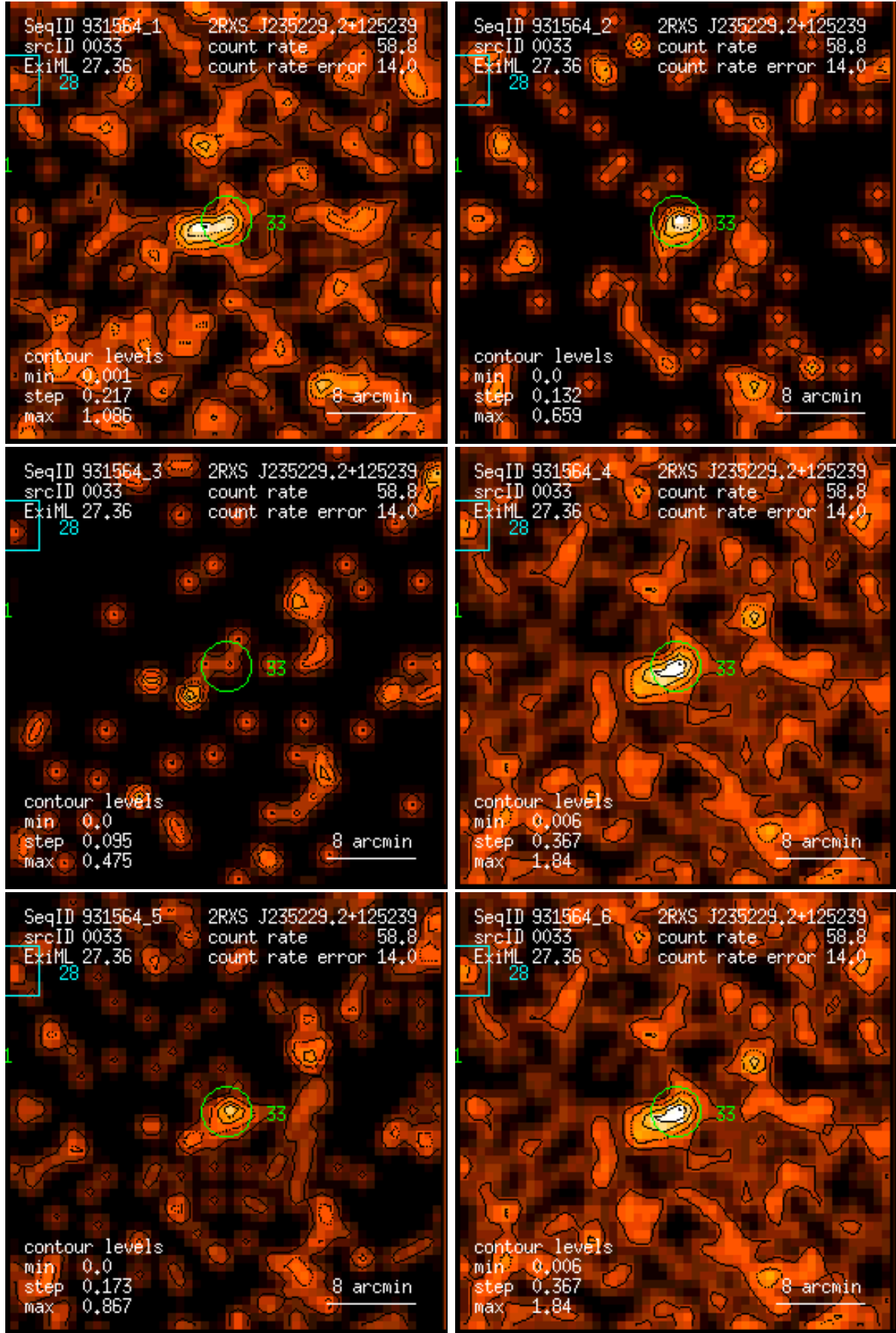
Figure 33: RASS 931564: detection 0033: band rate images, Gaussian filter: (1) PSPC channels 11 – 41, (2) 52 – 90, (3) 91 – 201, (4) 11 – 235, (5) 52 – 201, (6) 11 – 201. Broad band rates in counts/ks. Band rate contour levels in counts/ks/arcmin 2 .
