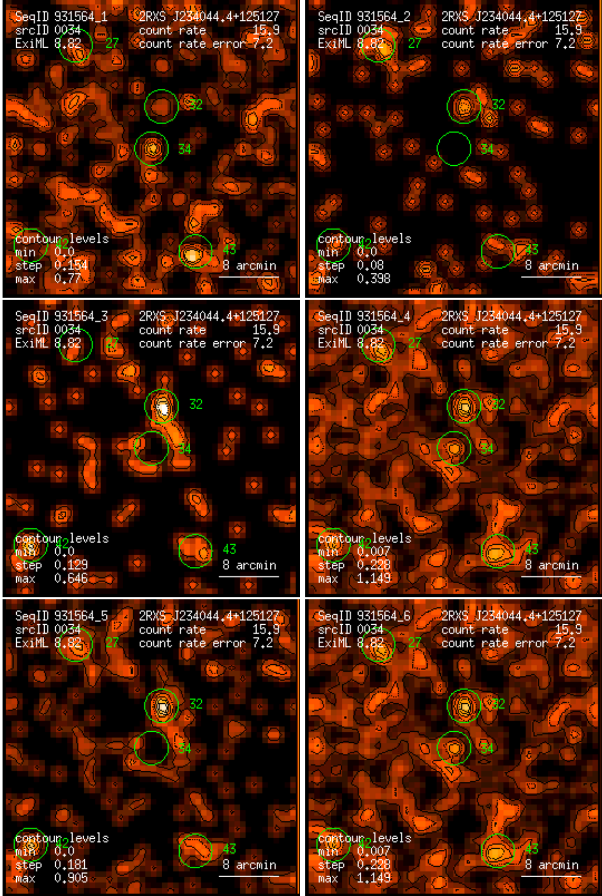
Figure 34: RASS 931564: detection 0034: band rate images, Gaussian filter: (1) PSPC channels 11 – 41, (2) 52 – 90, (3) 91 – 201, (4) 11 – 235, (5) 52 – 201, (6) 11 – 201. Broad band rates in counts/ks. Band rate contour levels in counts/ks/arcmin 2 .
