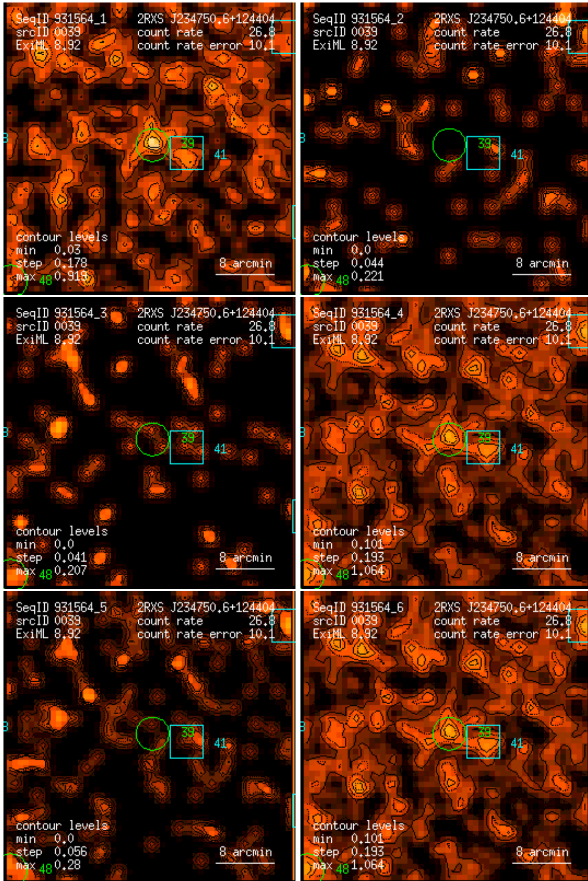
Figure 39: RASS 931564: detection 0039: band rate images, Gaussian filter: (1) PSPC channels 11 – 41, (2) 52 – 90, (3) 91 – 201, (4) 11 – 235, (5) 52 – 201, (6) 11 – 201. Broad band rates in counts/ks. Band rate contour levels in counts/ks/arcmin 2 .
