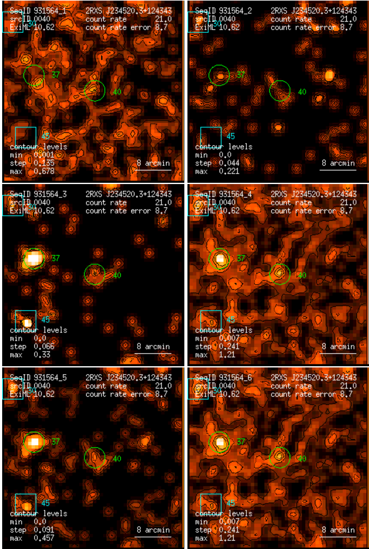
Figure 40: RASS 931564: detection 0040: band rate images, Gaussian filter: (1) PSPC channels 11 – 41, (2) 52 – 90, (3) 91 – 201, (4) 11 – 235, (5) 52 – 201, (6) 11 – 201. Broad band rates in counts/ks. Band rate contour levels in counts/ks/arcmin 2 .
