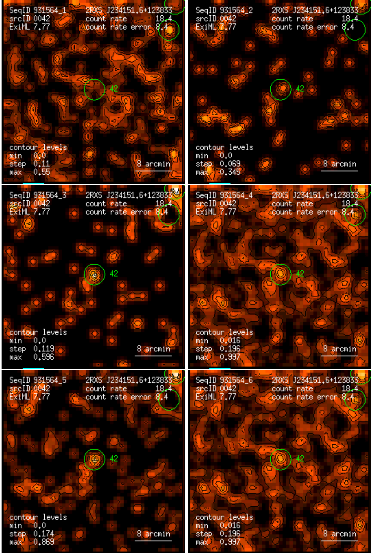
Figure 42: RASS 931564: detection 0042: band rate images, Gaussian filter: (1) PSPC channels 11 – 41, (2) 52 – 90, (3) 91 – 201, (4) 11 – 235, (5) 52 – 201, (6) 11 – 201. Broad band rates in counts/ks. Band rate contour levels in counts/ks/arcmin 2 .
