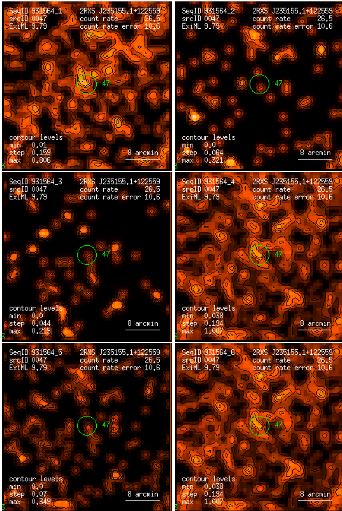
Figure 47: RASS 931564: detection 0047: band rate images, Gaussian filter: (1) PSPC channels 11 – 41, (2) 52 – 90, (3) 91 – 201, (4) 11 – 235, (5) 52 – 201, (6) 11 – 201. Broad band rates in counts/ks. Band rate contour levels in counts/ks/arcmin 2 .
