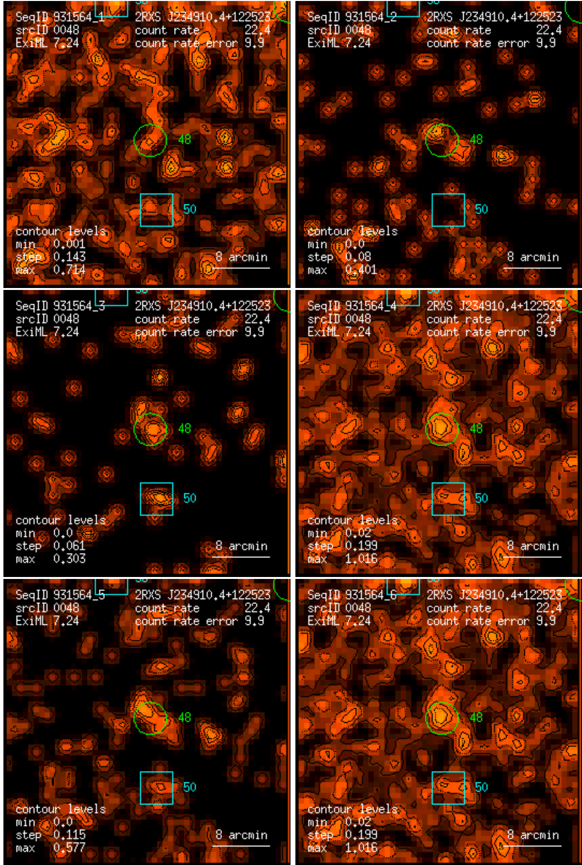
Figure 48: RASS 931564: detection 0048: band rate images, Gaussian filter: (1) PSPC channels 11 – 41, (2) 52 – 90, (3) 91 – 201, (4) 11 – 235, (5) 52 – 201, (6) 11 – 201. Broad band rates in counts/ks. Band rate contour levels in counts/ks/arcmin 2 .
