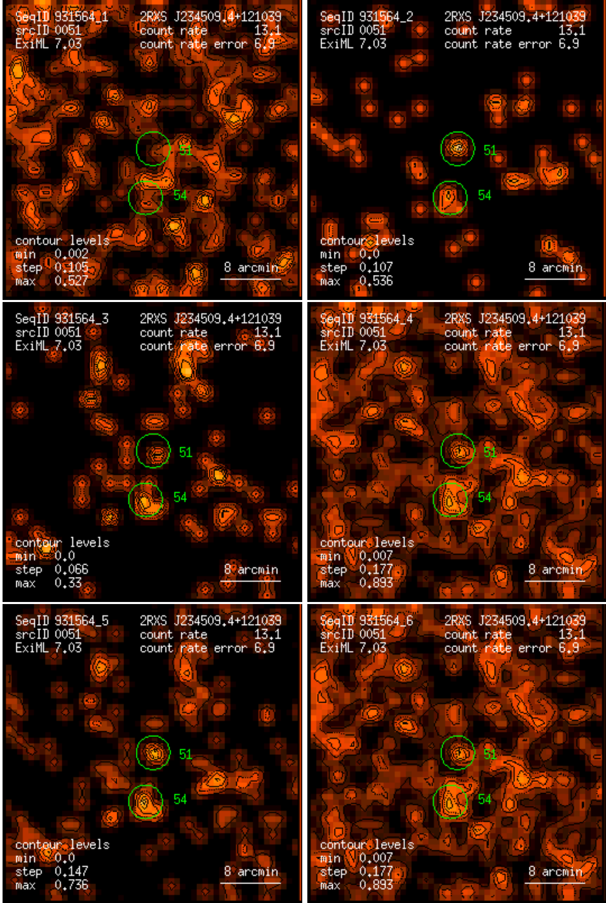
Figure 51: RASS 931564: detection 0051: band rate images, Gaussian filter: (1) PSPC channels 11 – 41, (2) 52 – 90, (3) 91 – 201, (4) 11 – 235, (5) 52 – 201, (6) 11 – 201. Broad band rates in counts/ks. Band rate contour levels in counts/ks/arcmin 2 .
