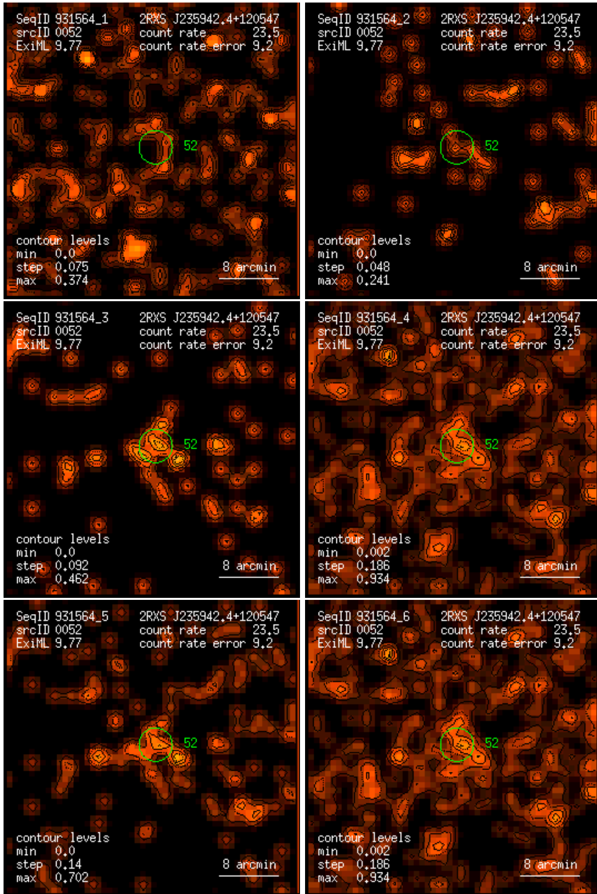
Figure 52: RASS 931564: detection 0052: band rate images, Gaussian filter: (1) PSPC channels 11 – 41, (2) 52 – 90, (3) 91 – 201, (4) 11 – 235, (5) 52 – 201, (6) 11 – 201. Broad band rates in counts/ks. Band rate contour levels in counts/ks/arcmin 2 .
