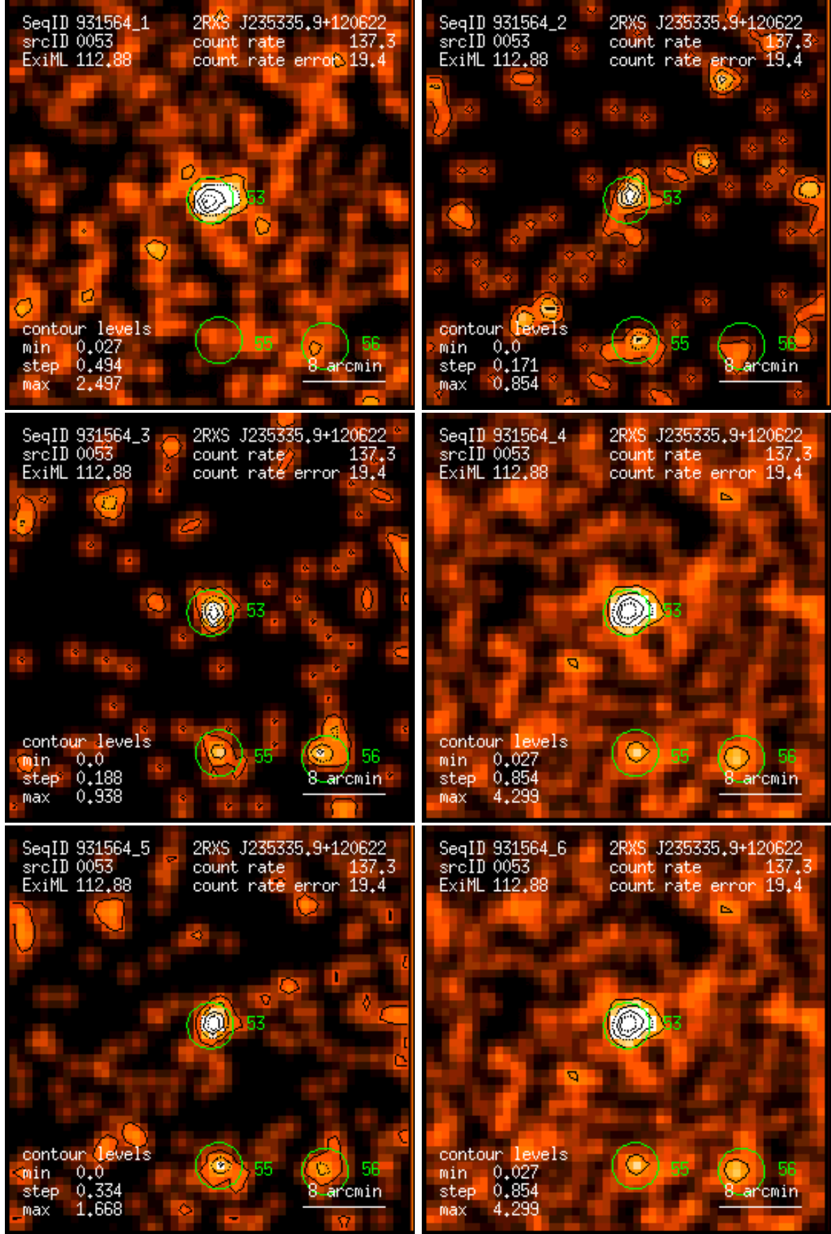
Figure 53: RASS 931564: detection 0053: band rate images, Gaussian filter: (1) PSPC channels 11 – 41, (2) 52 – 90, (3) 91 – 201, (4) 11 – 235, (5) 52 – 201, (6) 11 – 201. Broad band rates in counts/ks. Band rate contour levels in counts/ks/arcmin 2 .
