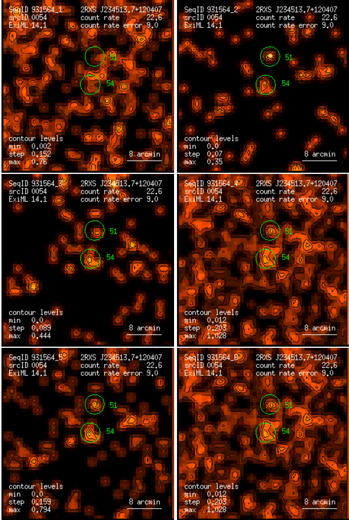
Figure 54: RASS 931564: detection 0054: band rate images, Gaussian filter: (1) PSPC channels 11 – 41, (2) 52 – 90, (3) 91 – 201, (4) 11 – 235, (5) 52 – 201, (6) 11 – 201. Broad band rates in counts/ks. Band rate contour levels in counts/ks/arcmin 2 .
