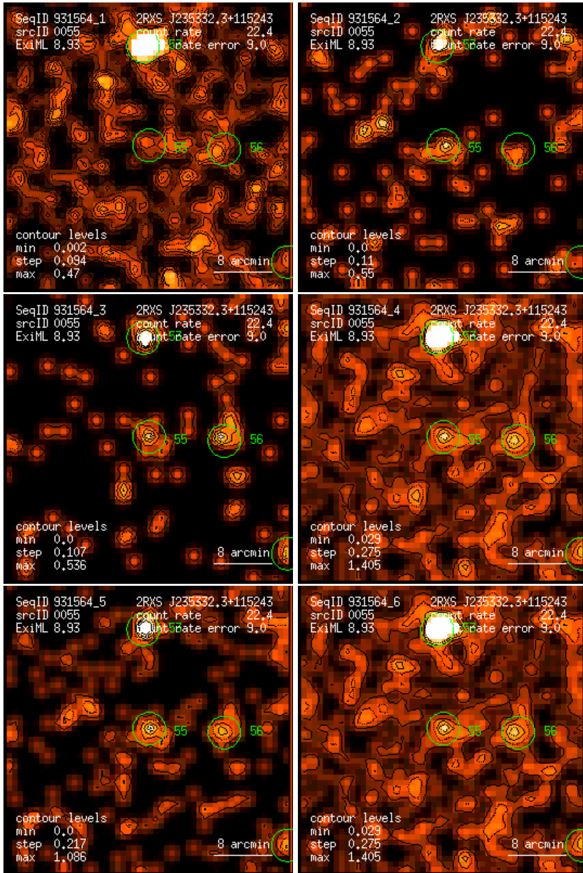
Figure 55: RASS 931564: detection 0055: band rate images, Gaussian filter: (1) PSPC channels 11 – 41, (2) 52 – 90, (3) 91 – 201, (4) 11 – 235, (5) 52 – 201, (6) 11 – 201. Broad band rates in counts/ks. Band rate contour levels in counts/ks/arcmin 2 .
