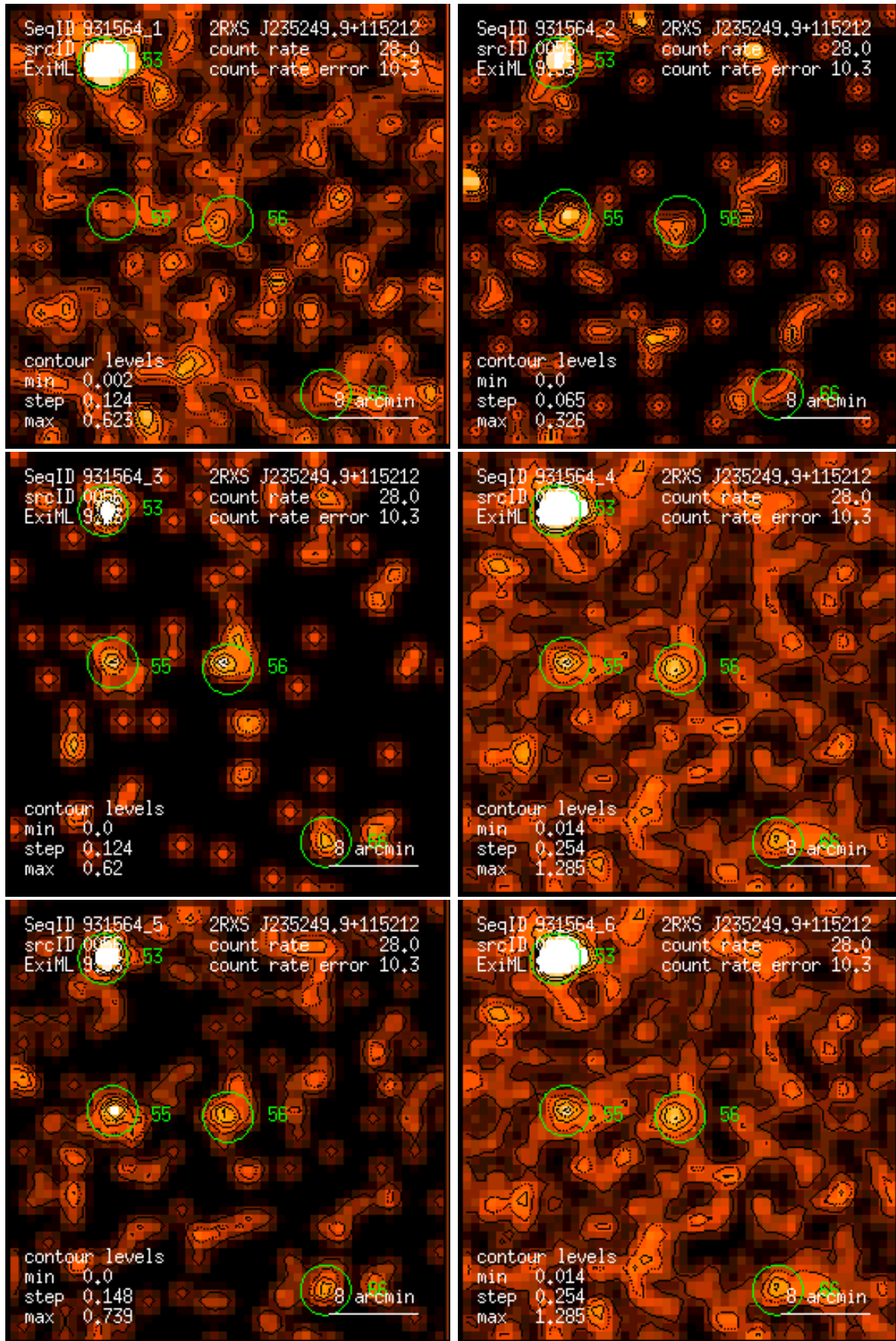
Figure 56: RASS 931564: detection 0056: band rate images, Gaussian filter: (1) PSPC channels 11 – 41, (2) 52 – 90, (3) 91 – 201, (4) 11 – 235, (5) 52 – 201, (6) 11 – 201. Broad band rates in counts/ks. Band rate contour levels in counts/ks/arcmin 2 .
