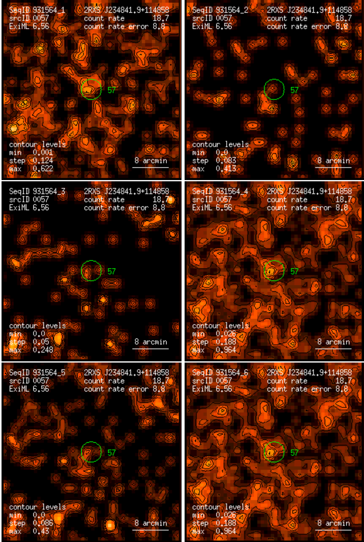
Figure 57: RASS 931564: detection 0057: band rate images, Gaussian filter: (1) PSPC channels 11 – 41, (2) 52 – 90, (3) 91 – 201, (4) 11 – 235, (5) 52 – 201, (6) 11 – 201. Broad band rates in counts/ks. Band rate contour levels in counts/ks/arcmin 2 .
