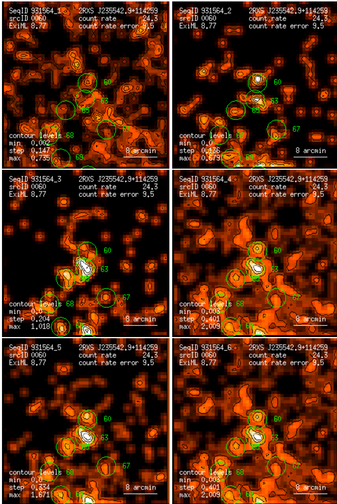
Figure 60: RASS 931564: detection 0060: band rate images, Gaussian filter: (1) PSPC channels 11 – 41, (2) 52 – 90, (3) 91 – 201, (4) 11 – 235, (5) 52 – 201, (6) 11 – 201. Broad band rates in counts/ks. Band rate contour levels in counts/ks/arcmin 2 .
