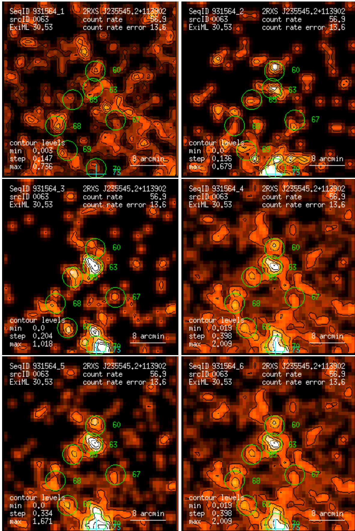
Figure 63: RASS 931564: detection 0063: band rate images, Gaussian filter: (1) PSPC channels 11 – 41, (2) 52 – 90, (3) 91 – 201, (4) 11 – 235, (5) 52 – 201, (6) 11 – 201. Broad band rates in counts/ks. Band rate contour levels in counts/ks/arcmin 2 .
