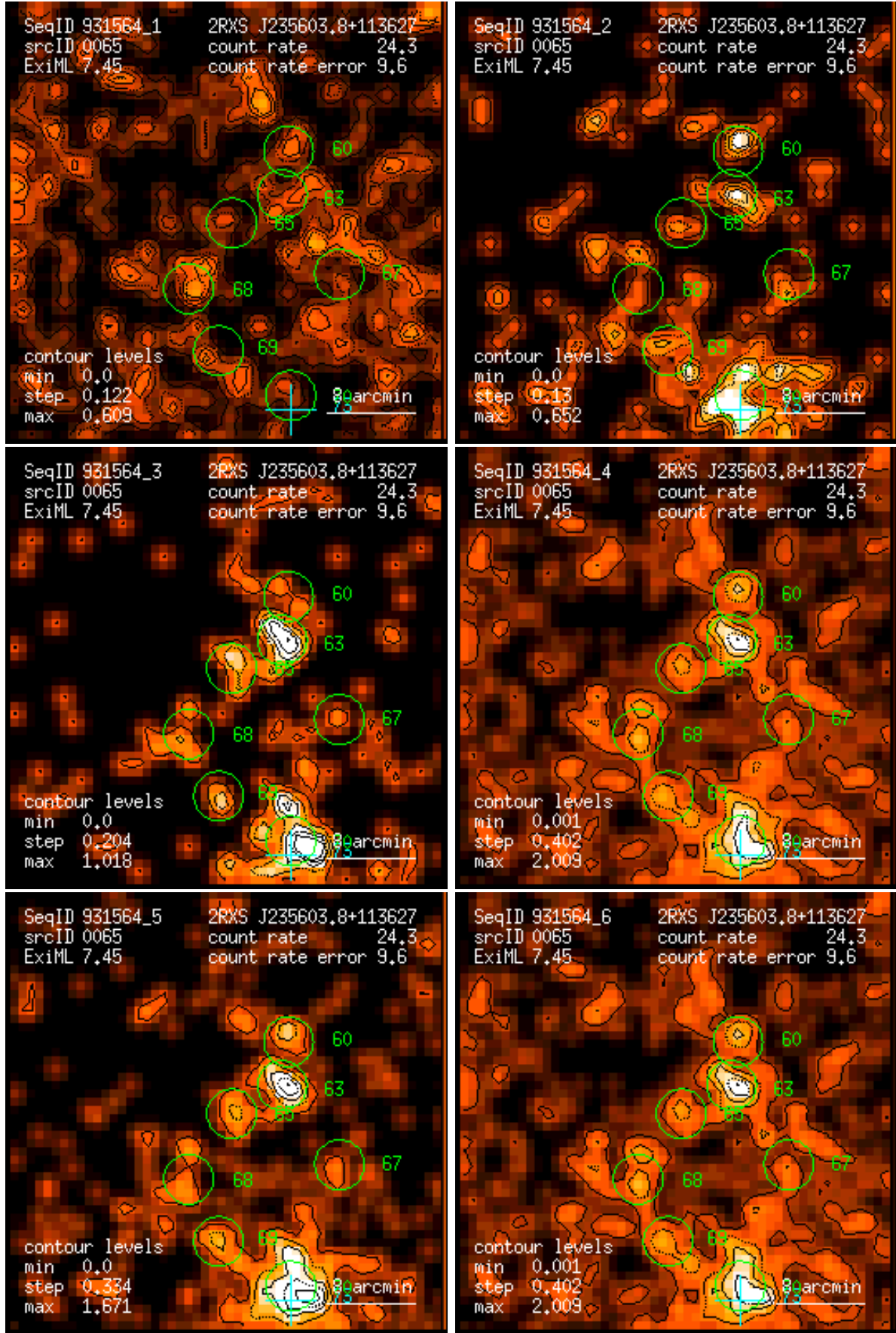
Figure 65: RASS 931564: detection 0065: band rate images, Gaussian filter: (1) PSPC channels 11 – 41, (2) 52 – 90, (3) 91 – 201, (4) 11 – 235, (5) 52 – 201, (6) 11 – 201. Broad band rates in counts/ks. Band rate contour levels in counts/ks/arcmin 2 .
