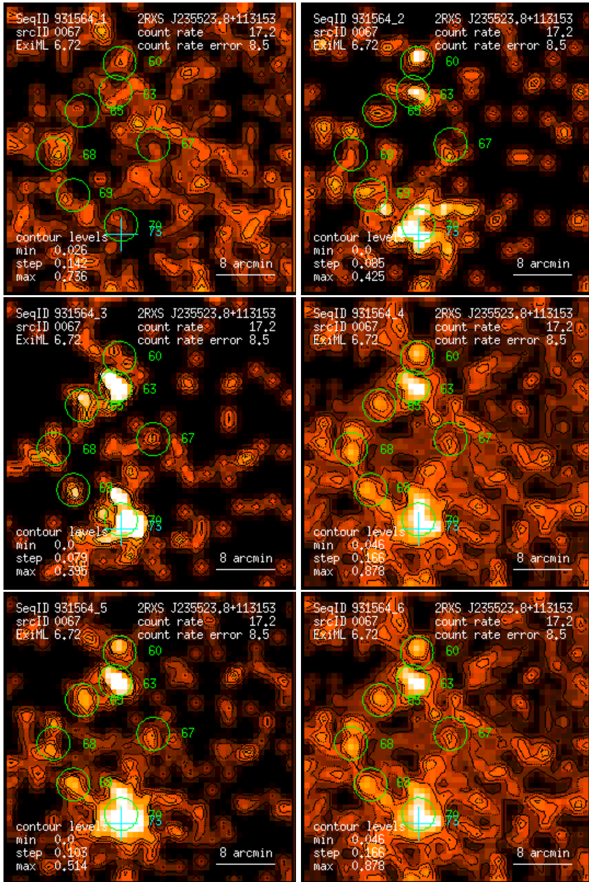
Figure 67: RASS 931564: detection 0067: band rate images, Gaussian filter: (1) PSPC channels 11 – 41, (2) 52 – 90, (3) 91 – 201, (4) 11 – 235, (5) 52 – 201, (6) 11 – 201. Broad band rates in counts/ks. Band rate contour levels in counts/ks/arcmin 2 .
