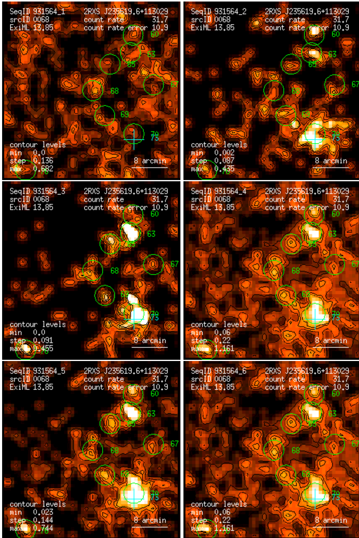
Figure 68: RASS 931564: detection 0068: band rate images, Gaussian filter: (1) PSPC channels 11 – 41, (2) 52 – 90, (3) 91 – 201, (4) 11 – 235, (5) 52 – 201, (6) 11 – 201. Broad band rates in counts/ks. Band rate contour levels in counts/ks/arcmin 2 .
