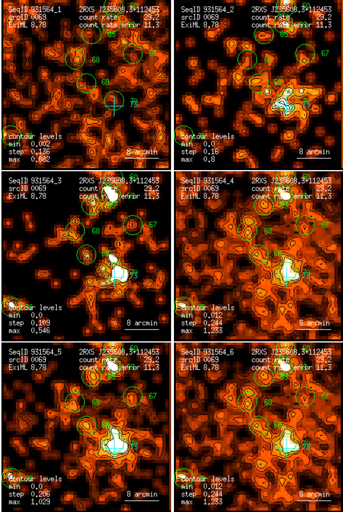
Figure 69: RASS 931564: detection 0069: band rate images, Gaussian filter: (1) PSPC channels 11 – 41, (2) 52 – 90, (3) 91 – 201, (4) 11 – 235, (5) 52 – 201, (6) 11 – 201. Broad band rates in counts/ks. Band rate contour levels in counts/ks/arcmin 2 .
