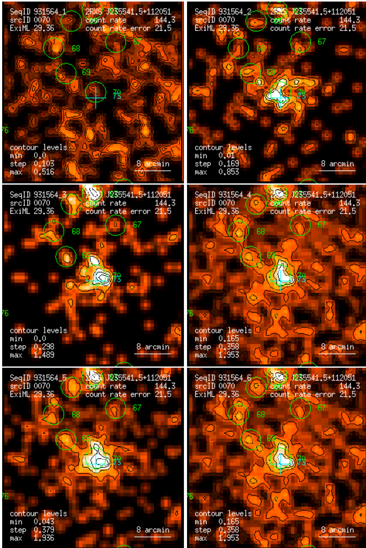
Figure 70: RASS 931564: detection 0070: band rate images, Gaussian filter: (1) PSPC channels 11 – 41, (2) 52 – 90, (3) 91 – 201, (4) 11 – 235, (5) 52 – 201, (6) 11 – 201. Broad band rates in counts/ks. Band rate contour levels in counts/ks/arcmin 2 .
