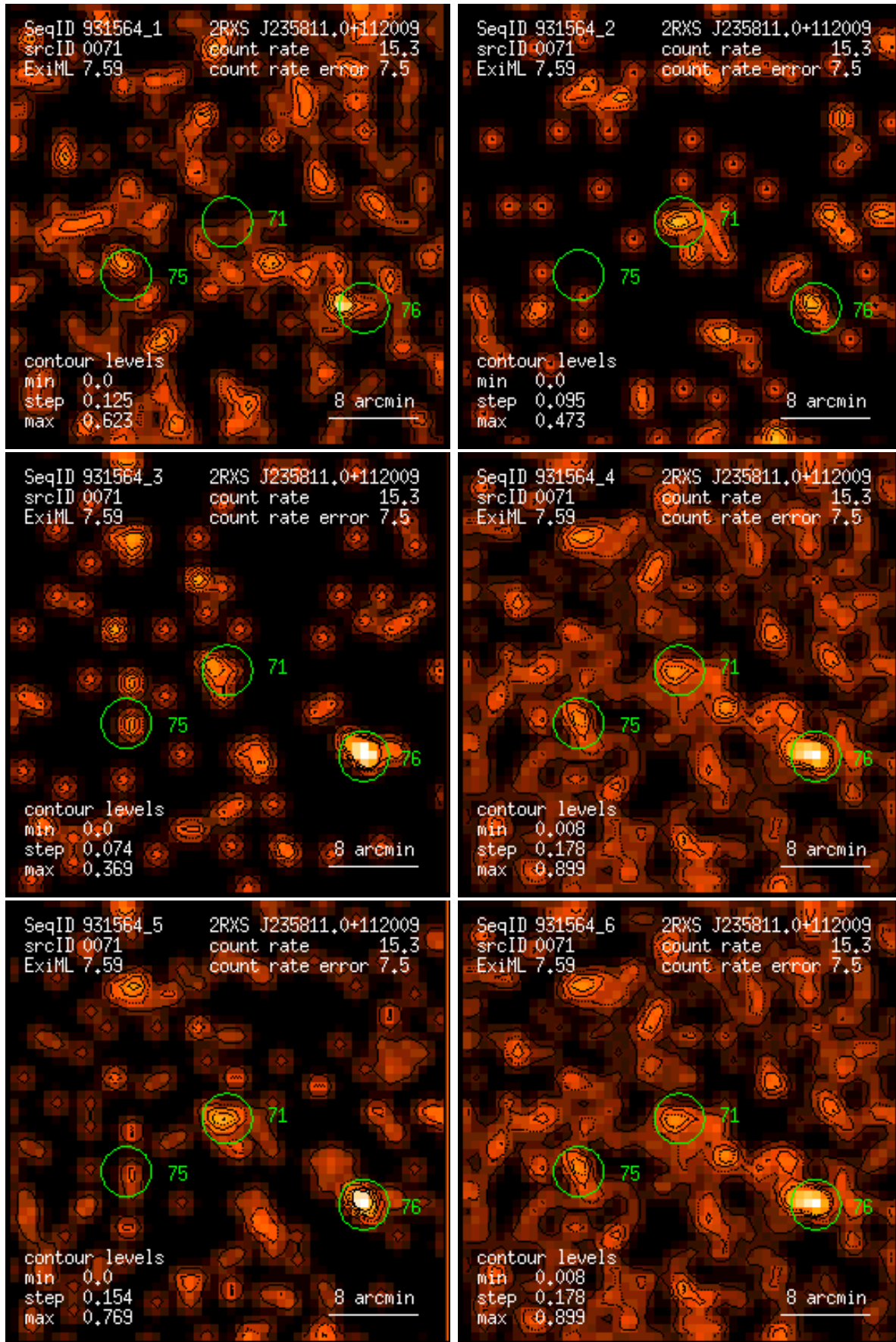
Figure 71: RASS 931564: detection 0071: band rate images, Gaussian filter: (1) PSPC channels 11 – 41, (2) 52 – 90, (3) 91 – 201, (4) 11 – 235, (5) 52 – 201, (6) 11 – 201. Broad band rates in counts/ks. Band rate contour levels in counts/ks/arcmin 2 .
