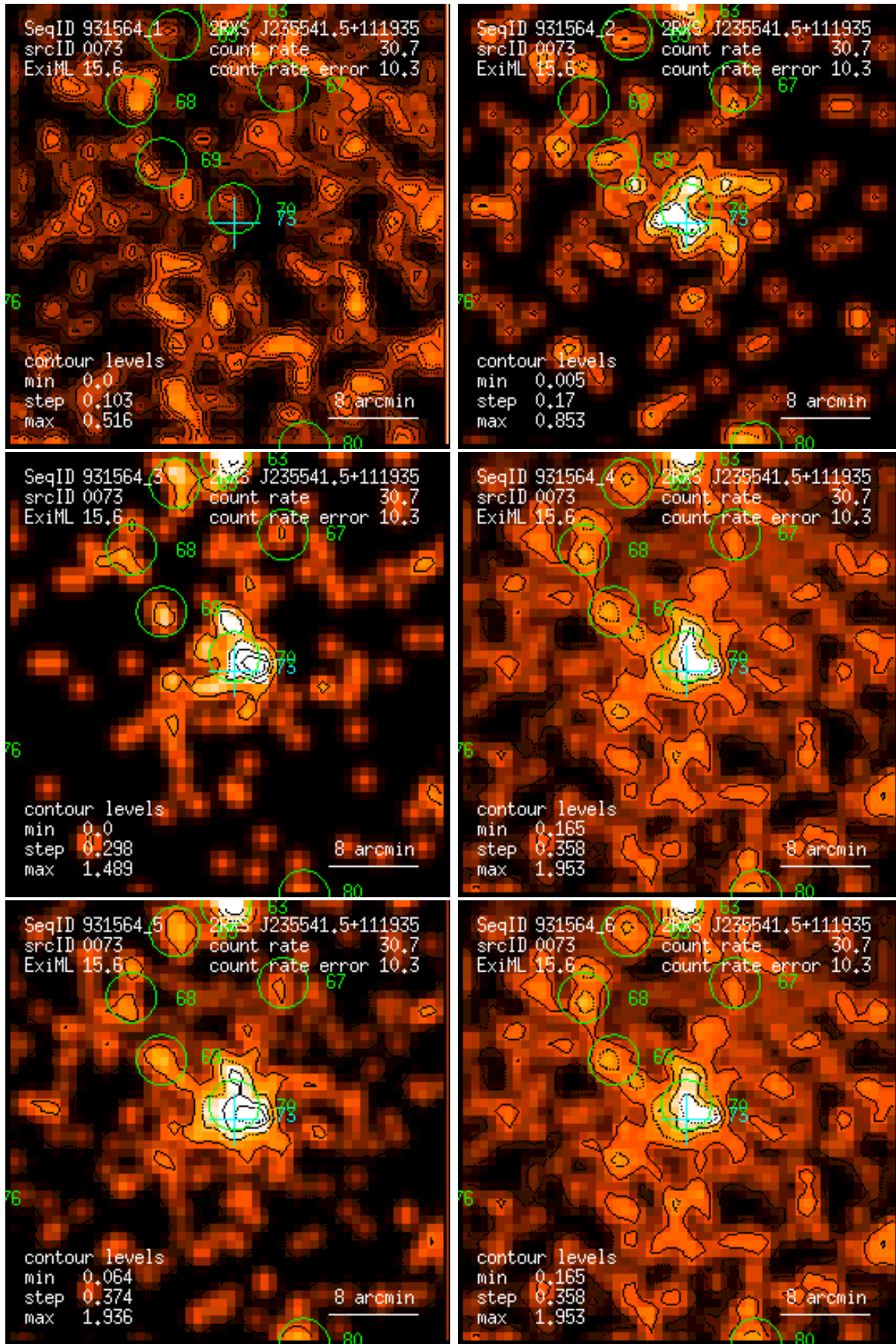
Figure 73: RASS 931564: detection 0073: band rate images, Gaussian filter: (1) PSPC channels 11 – 41, (2) 52 – 90, (3) 91 – 201, (4) 11 – 235, (5) 52 – 201, (6) 11 – 201. Broad band rates in counts/ks. Band rate contour levels in counts/ks/arcmin 2 .
