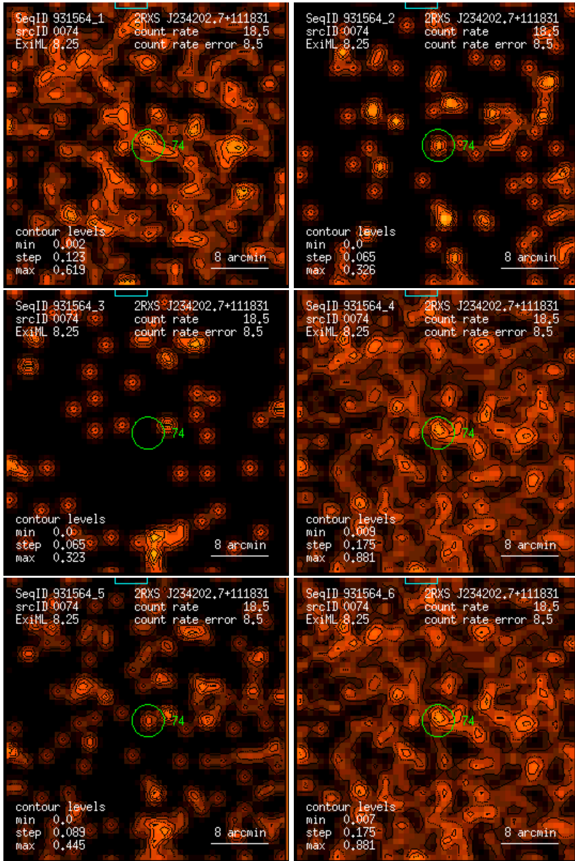
Figure 74: RASS 931564: detection 0074: band rate images, Gaussian filter: (1) PSPC channels 11 – 41, (2) 52 – 90, (3) 91 – 201, (4) 11 – 235, (5) 52 – 201, (6) 11 – 201. Broad band rates in counts/ks. Band rate contour levels in counts/ks/arcmin 2 .
