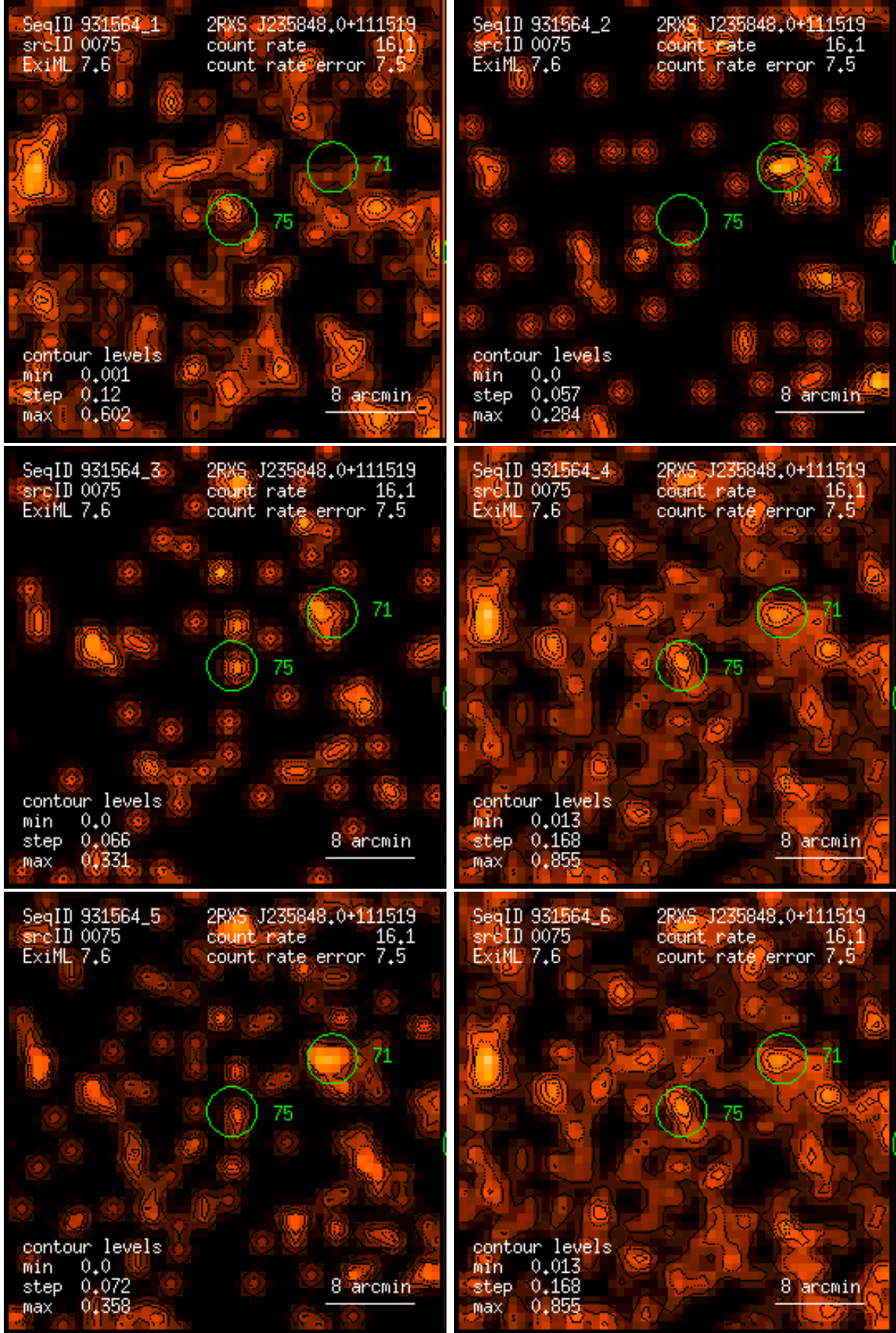
Figure 75: RASS 931564: detection 0075: band rate images, Gaussian filter: (1) PSPC channels 11 – 41, (2) 52 – 90, (3) 91 – 201, (4) 11 – 235, (5) 52 – 201, (6) 11 – 201. Broad band rates in counts/ks. Band rate contour levels in counts/ks/arcmin 2 .
