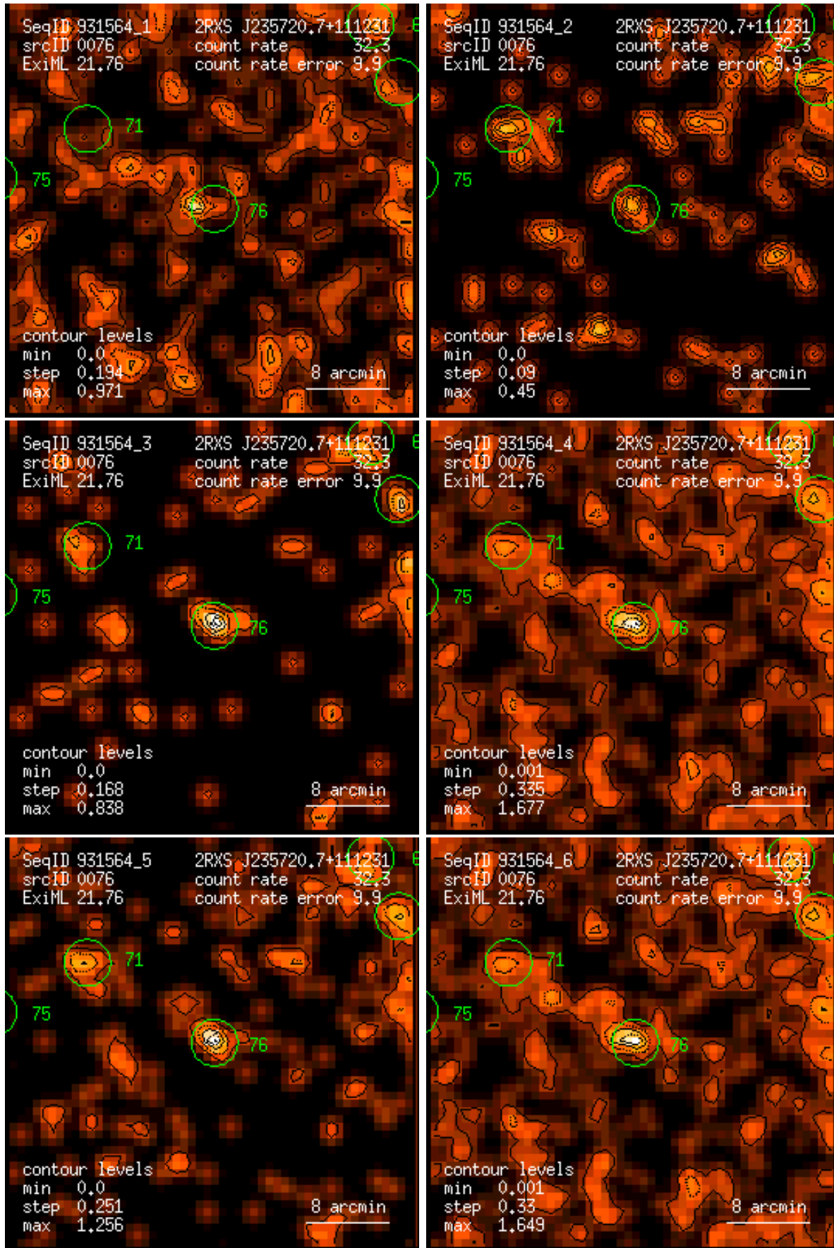
Figure 76: RASS 931564: detection 0076: band rate images, Gaussian filter: (1) PSPC channels 11 – 41, (2) 52 – 90, (3) 91 – 201, (4) 11 – 235, (5) 52 – 201, (6) 11 – 201. Broad band rates in counts/ks. Band rate contour levels in counts/ks/arcmin 2 .
