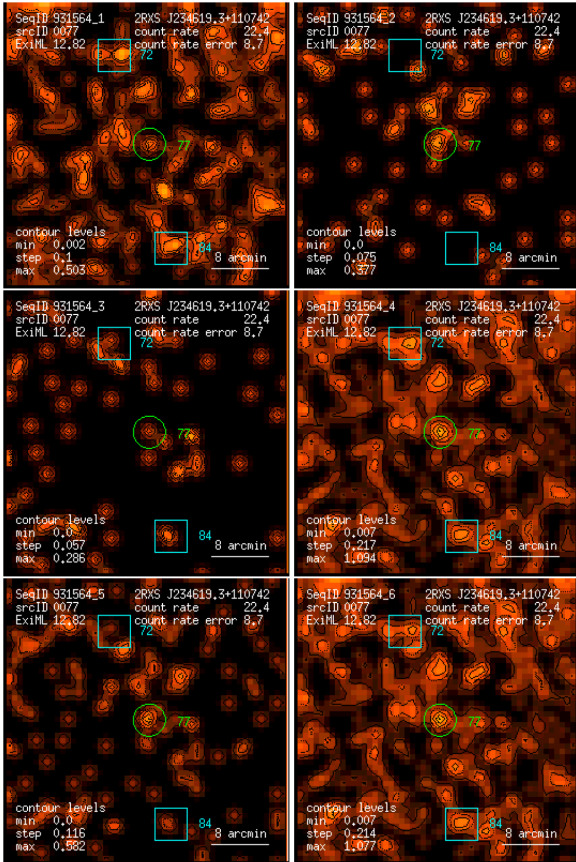
Figure 77: RASS 931564: detection 0077: band rate images, Gaussian filter: (1) PSPC channels 11 – 41, (2) 52 – 90, (3) 91 – 201, (4) 11 – 235, (5) 52 – 201, (6) 11 – 201. Broad band rates in counts/ks. Band rate contour levels in counts/ks/arcmin 2 .
