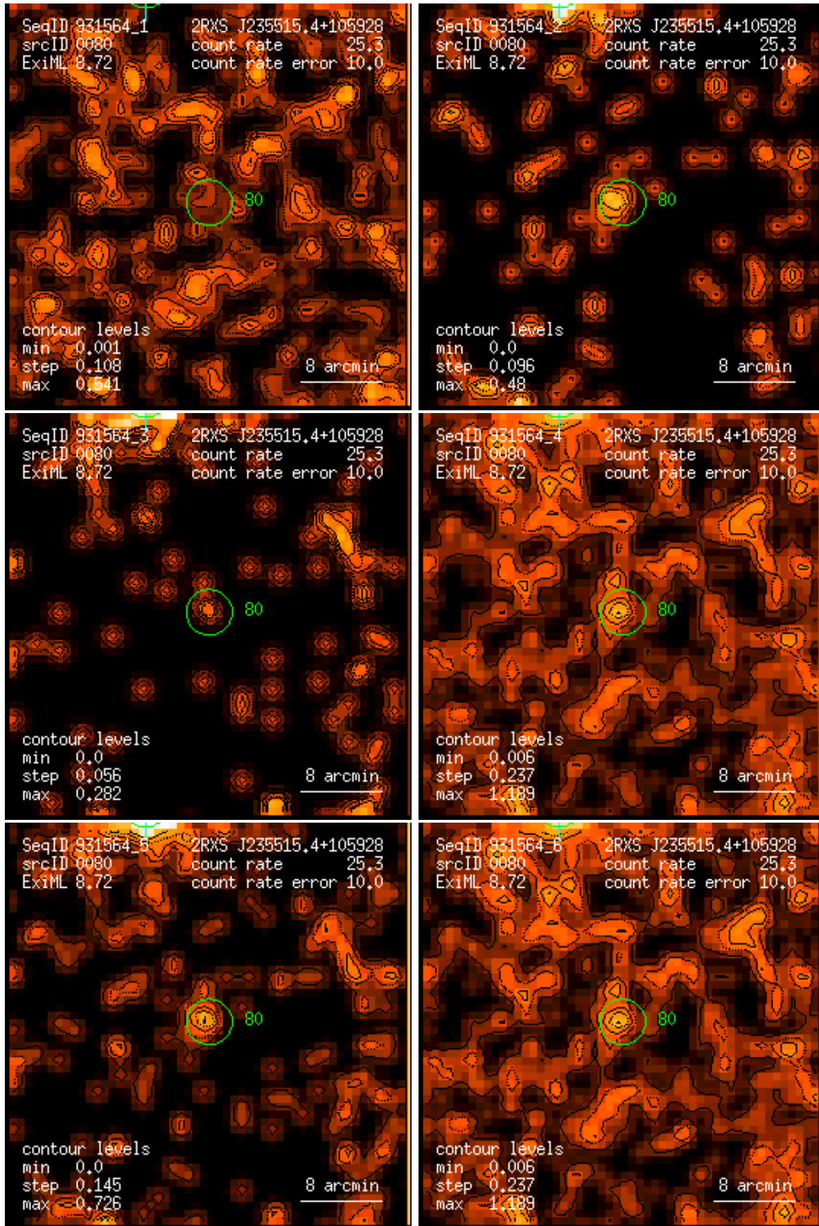
Figure 80: RASS 931564: detection 0080: band rate images, Gaussian filter: (1) PSPC channels 11 – 41, (2) 52 – 90, (3) 91 – 201, (4) 11 – 235, (5) 52 – 201, (6) 11 – 201. Broad band rates in counts/ks. Band rate contour levels in counts/ks/arcmin 2 .
