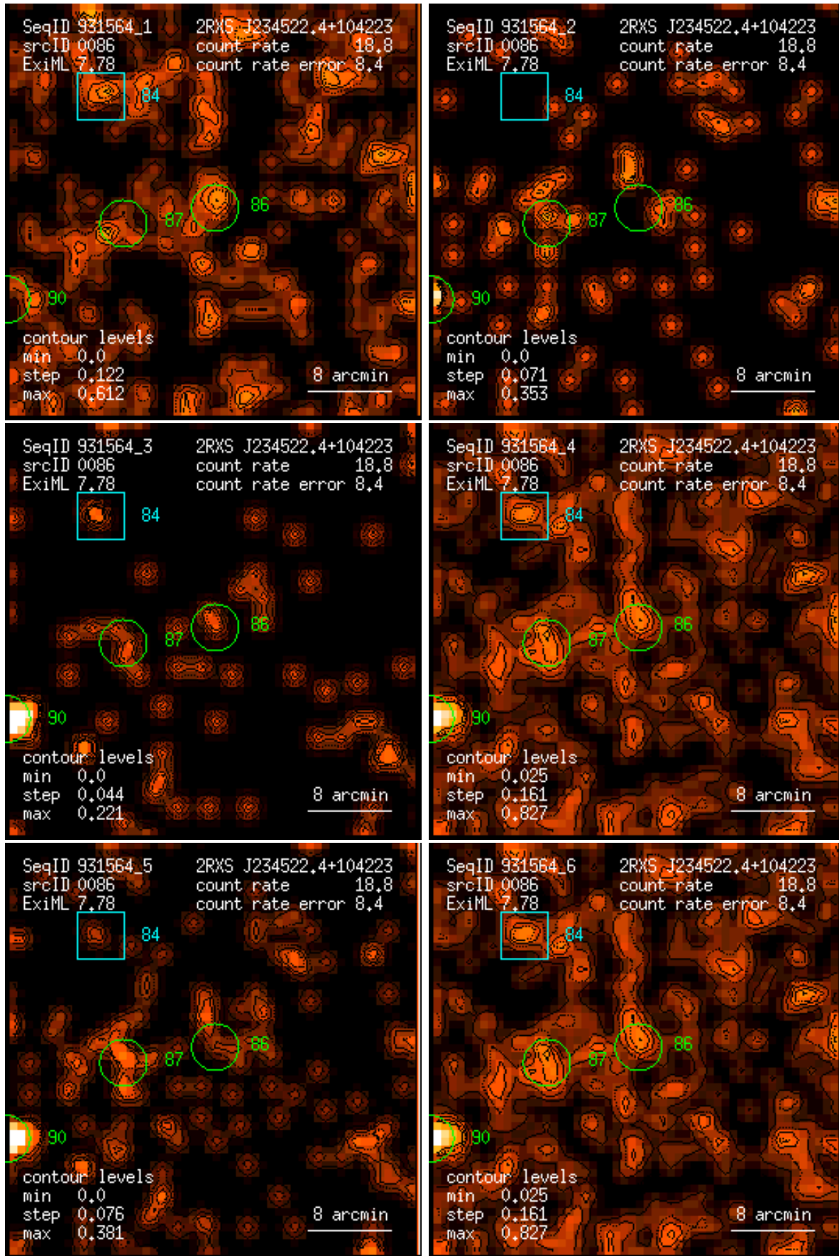
Figure 86: RASS 931564: detection 0086: band rate images, Gaussian filter: (1) PSPC channels 11 – 41, (2) 52 – 90, (3) 91 – 201, (4) 11 – 235, (5) 52 – 201, (6) 11 – 201. Broad band rates in counts/ks. Band rate contour levels in counts/ks/arcmin 2 .
