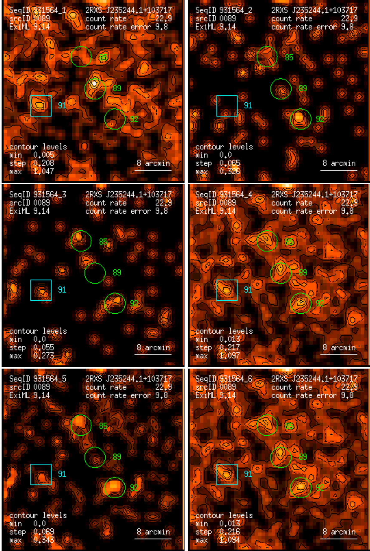
Figure 89: RASS 931564: detection 0089: band rate images, Gaussian filter: (1) PSPC channels 11 – 41, (2) 52 – 90, (3) 91 – 201, (4) 11 – 235, (5) 52 – 201, (6) 11 – 201. Broad band rates in counts/ks. Band rate contour levels in counts/ks/arcmin 2 .
