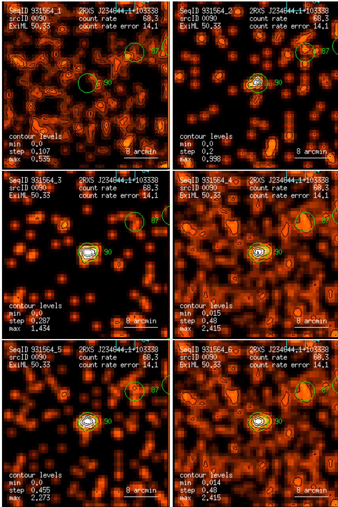
Figure 90: RASS 931564: detection 0090: band rate images, Gaussian filter: (1) PSPC channels 11 – 41, (2) 52 – 90, (3) 91 – 201, (4) 11 – 235, (5) 52 – 201, (6) 11 – 201. Broad band rates in counts/ks. Band rate contour levels in counts/ks/arcmin 2 .
