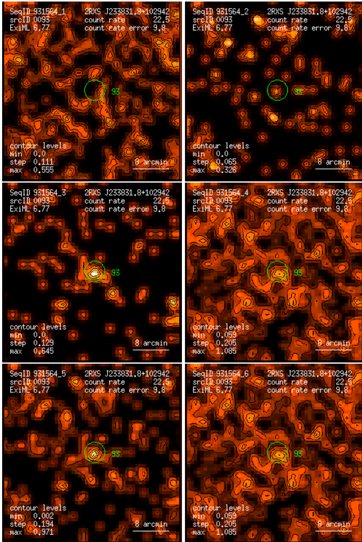
Figure 93: RASS 931564: detection 0093: band rate images, Gaussian filter: (1) PSPC channels 11 – 41, (2) 52 – 90, (3) 91 – 201, (4) 11 – 235, (5) 52 – 201, (6) 11 – 201. Broad band rates in counts/ks. Band rate contour levels in counts/ks/arcmin 2 .
