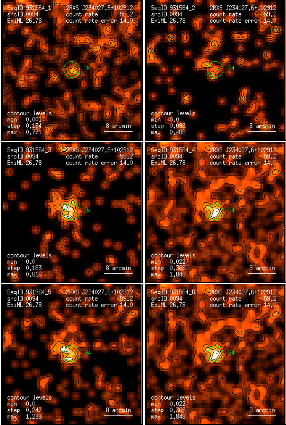
Figure 94: RASS 931564: detection 0094: band rate images, Gaussian filter: (1) PSPC channels 11 – 41, (2) 52 – 90, (3) 91 – 201, (4) 11 – 235, (5) 52 – 201, (6) 11 – 201. Broad band rates in counts/ks. Band rate contour levels in counts/ks/arcmin 2 .
