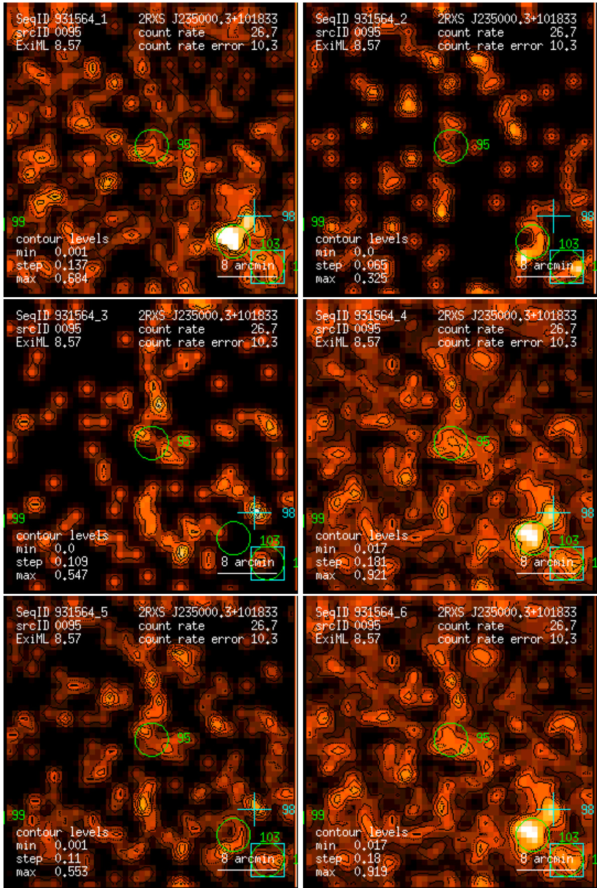
Figure 95: RASS 931564: detection 0095: band rate images, Gaussian filter: (1) PSPC channels 11 – 41, (2) 52 – 90, (3) 91 – 201, (4) 11 – 235, (5) 52 – 201, (6) 11 – 201. Broad band rates in counts/ks. Band rate contour levels in counts/ks/arcmin 2 .
