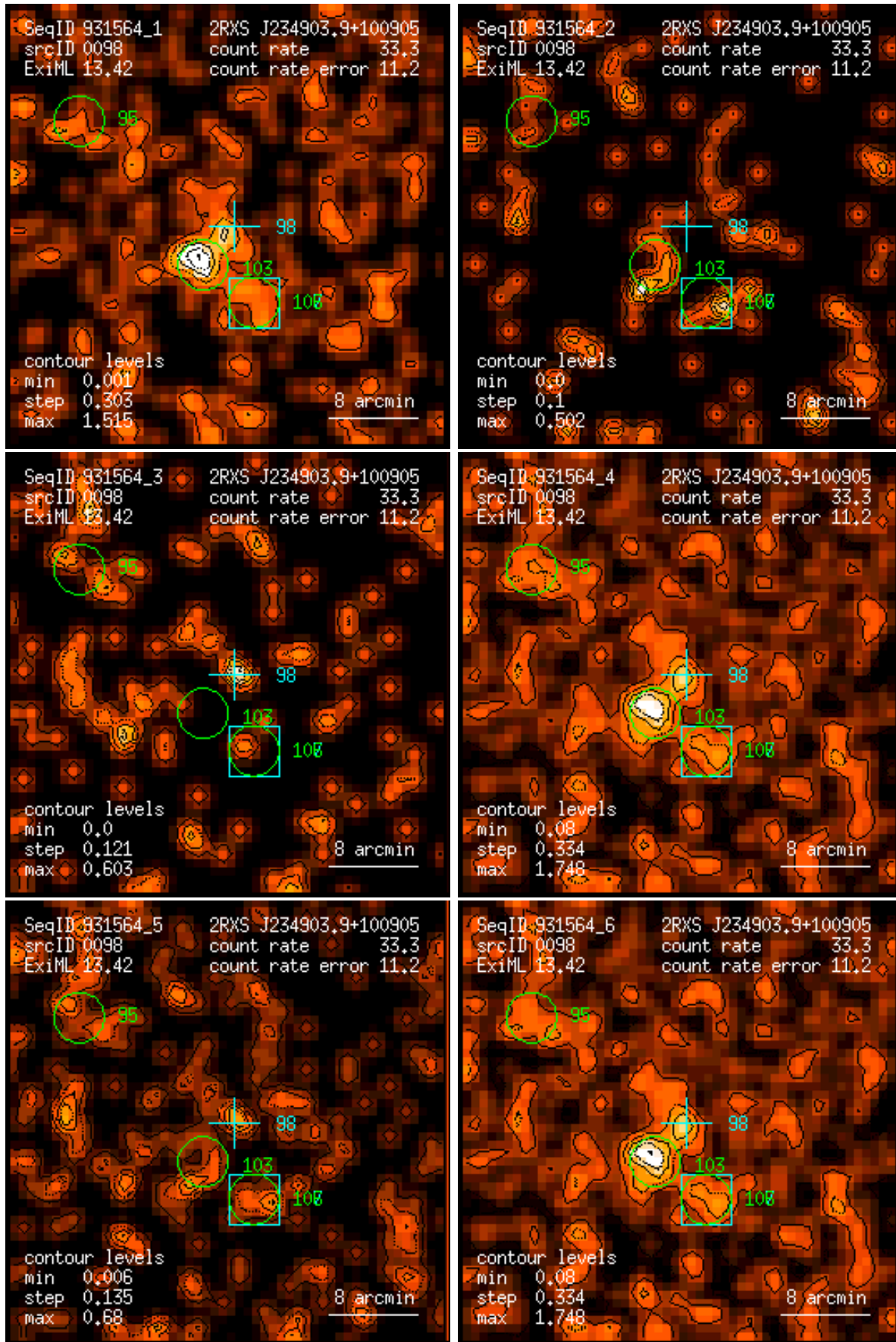
Figure 98: RASS 931564: detection 0098: band rate images, Gaussian filter: (1) PSPC channels 11 – 41, (2) 52 – 90, (3) 91 – 201, (4) 11 – 235, (5) 52 – 201, (6) 11 – 201. Broad band rates in counts/ks. Band rate contour levels in counts/ks/arcmin 2 .
