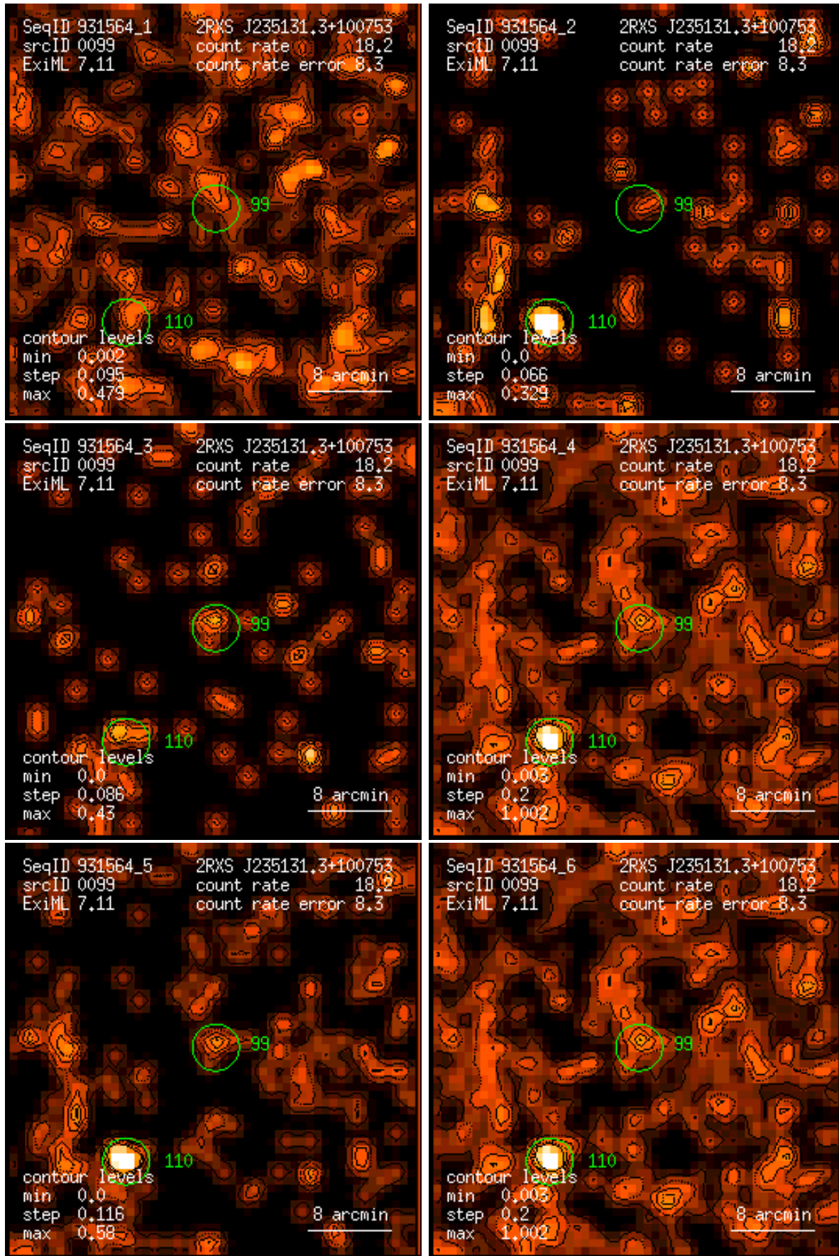
Figure 99: RASS 931564: detection 0099: band rate images, Gaussian filter: (1) PSPC channels 11 – 41, (2) 52 – 90, (3) 91 – 201, (4) 11 – 235, (5) 52 – 201, (6) 11 – 201. Broad band rates in counts/ks. Band rate contour levels in counts/ks/arcmin 2 .
