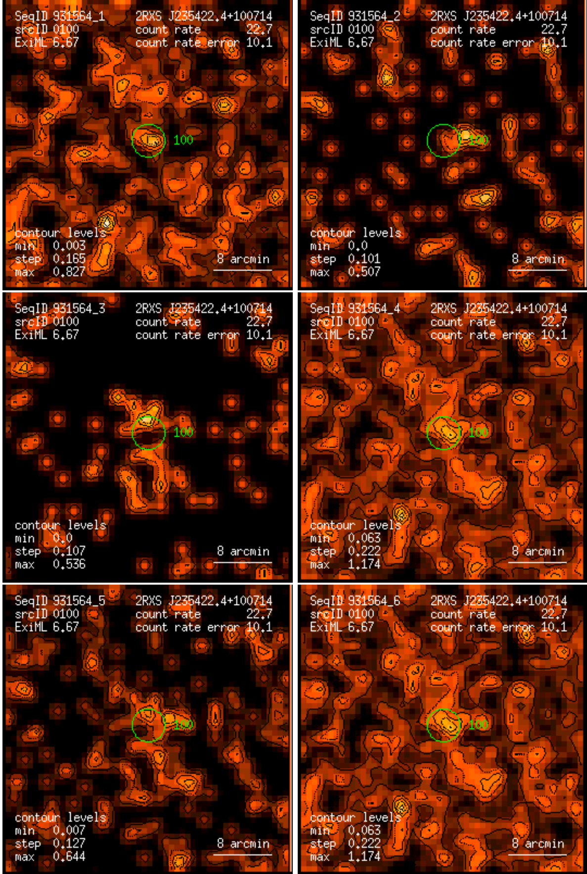
Figure 100: RASS 931564: detection 0100: band rate images, Gaussian filter: (1) PSPC channels 11 – 41, (2) 52 – 90, (3) 91 – 201, (4) 11 – 235, (5) 52 – 201, (6) 11 – 201. Broad band rates in counts/ks. Band rate contour levels in counts/ks/arcmin 2 .
