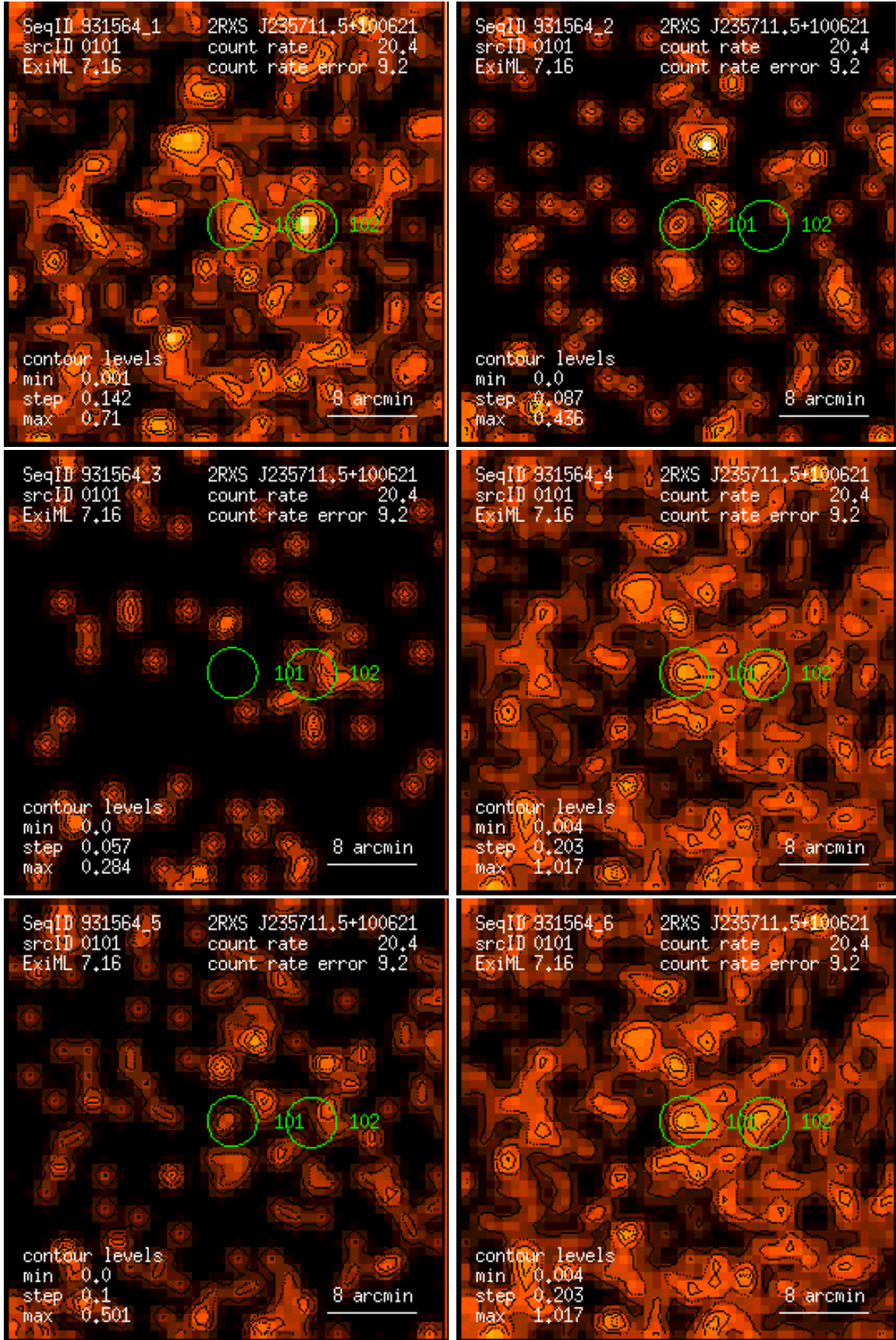
Figure 101: RASS 931564: detection 0101: band rate images, Gaussian filter: (1) PSPC channels 11 – 41, (2) 52 – 90, (3) 91 – 201, (4) 11 – 235, (5) 52 – 201, (6) 11 – 201. Broad band rates in counts/ks. Band rate contour levels in counts/ks/arcmin 2 .
