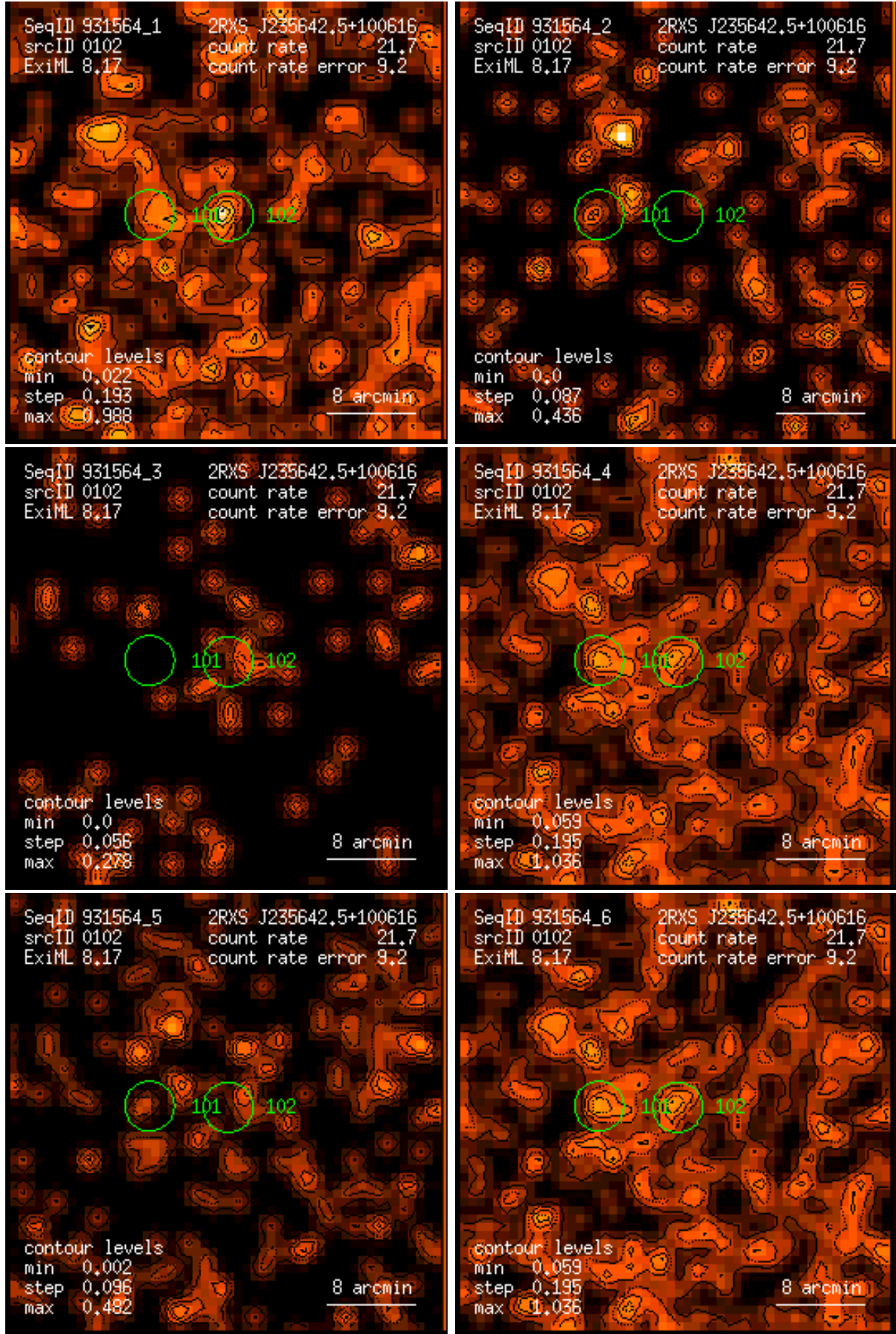
Figure 102: RASS 931564: detection 0102: band rate images, Gaussian filter: (1) PSPC channels 11 – 41, (2) 52 – 90, (3) 91 – 201, (4) 11 – 235, (5) 52 – 201, (6) 11 – 201. Broad band rates in counts/ks. Band rate contour levels in counts/ks/arcmin 2 .
