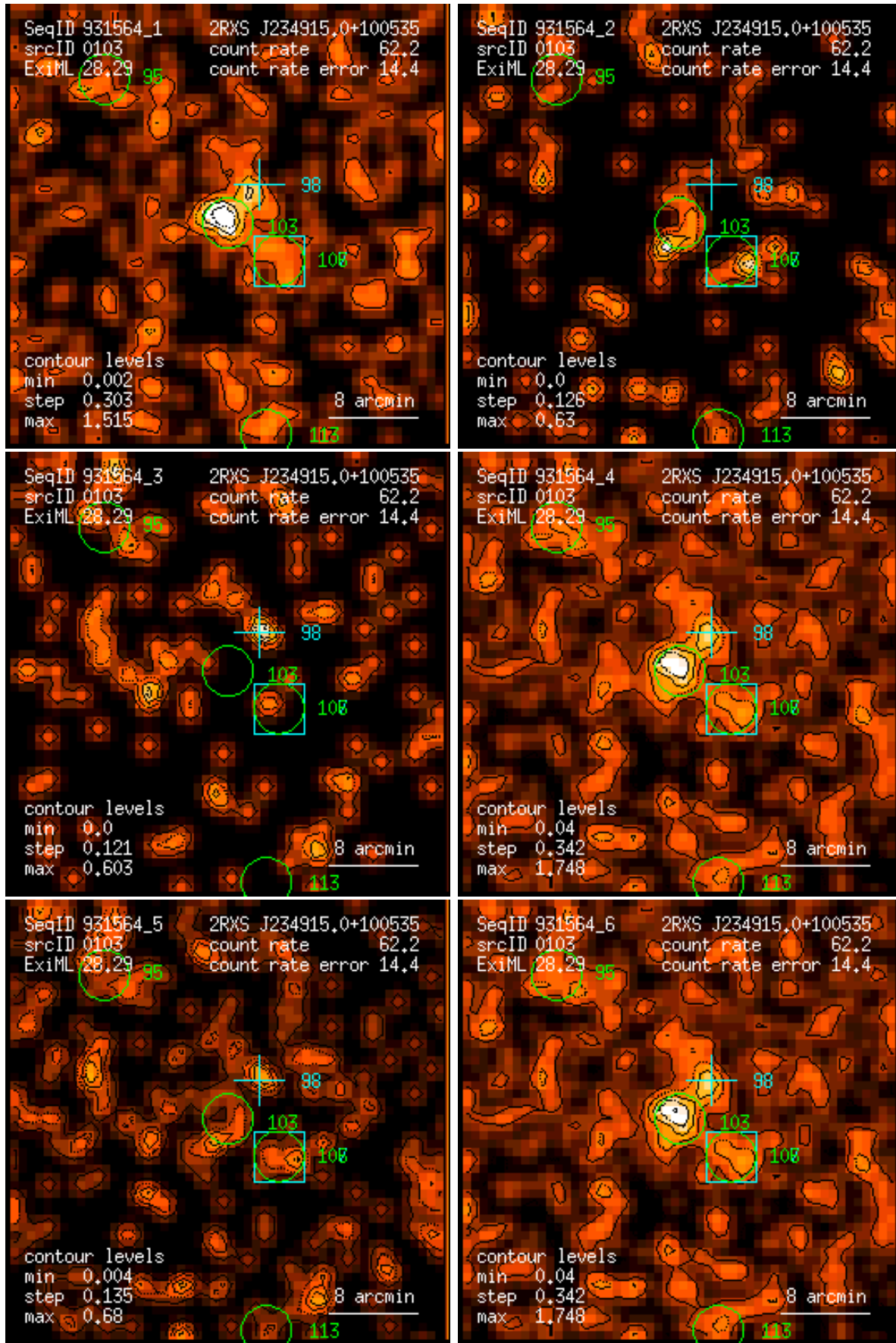
Figure 103: RASS 931564: detection 0103: band rate images, Gaussian filter: (1) PSPC channels 11 – 41, (2) 52 – 90, (3) 91 – 201, (4) 11 – 235, (5) 52 – 201, (6) 11 – 201. Broad band rates in counts/ks. Band rate contour levels in counts/ks/arcmin 2 .
