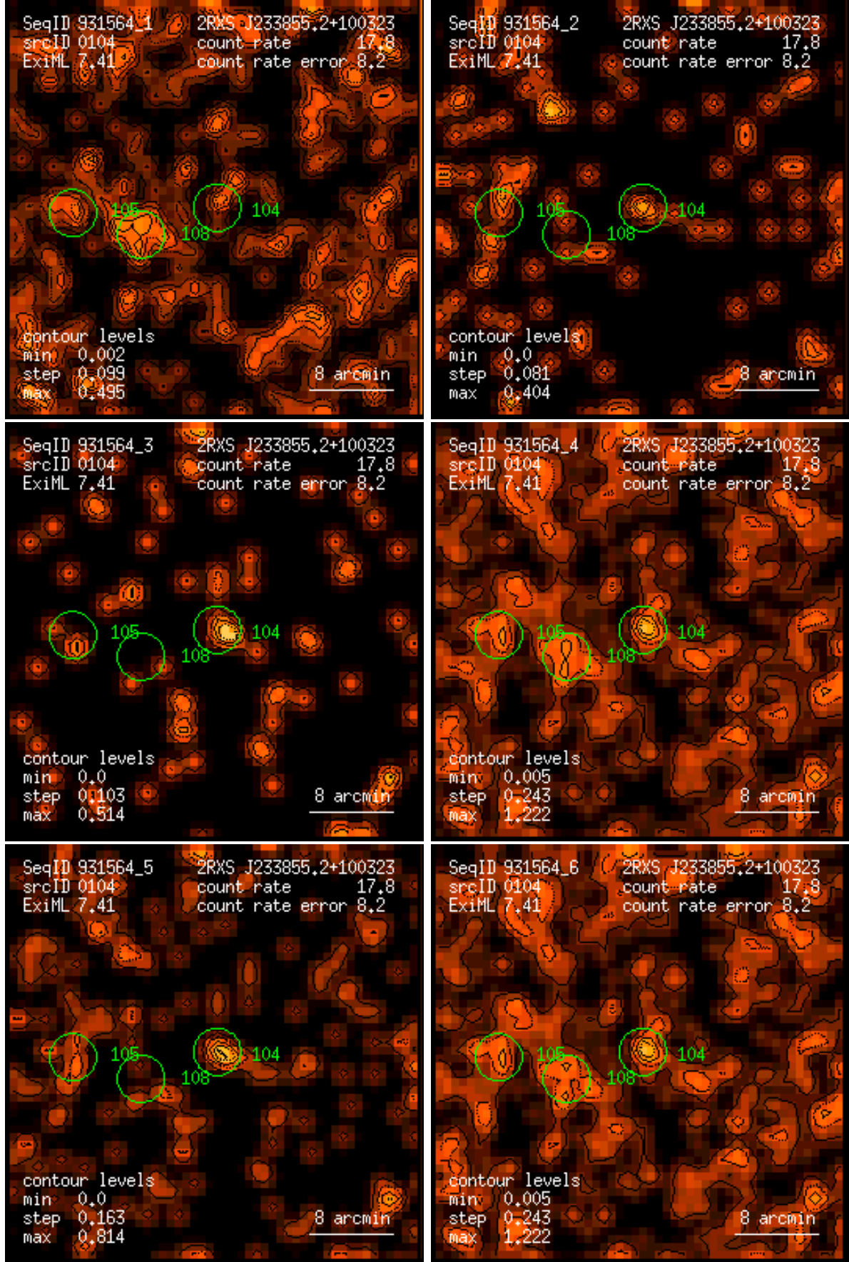
Figure 104: RASS 931564: detection 0104: band rate images, Gaussian filter: (1) PSPC channels 11 – 41, (2) 52 – 90, (3) 91 – 201, (4) 11 – 235, (5) 52 – 201, (6) 11 – 201. Broad band rates in counts/ks. Band rate contour levels in counts/ks/arcmin 2 .
