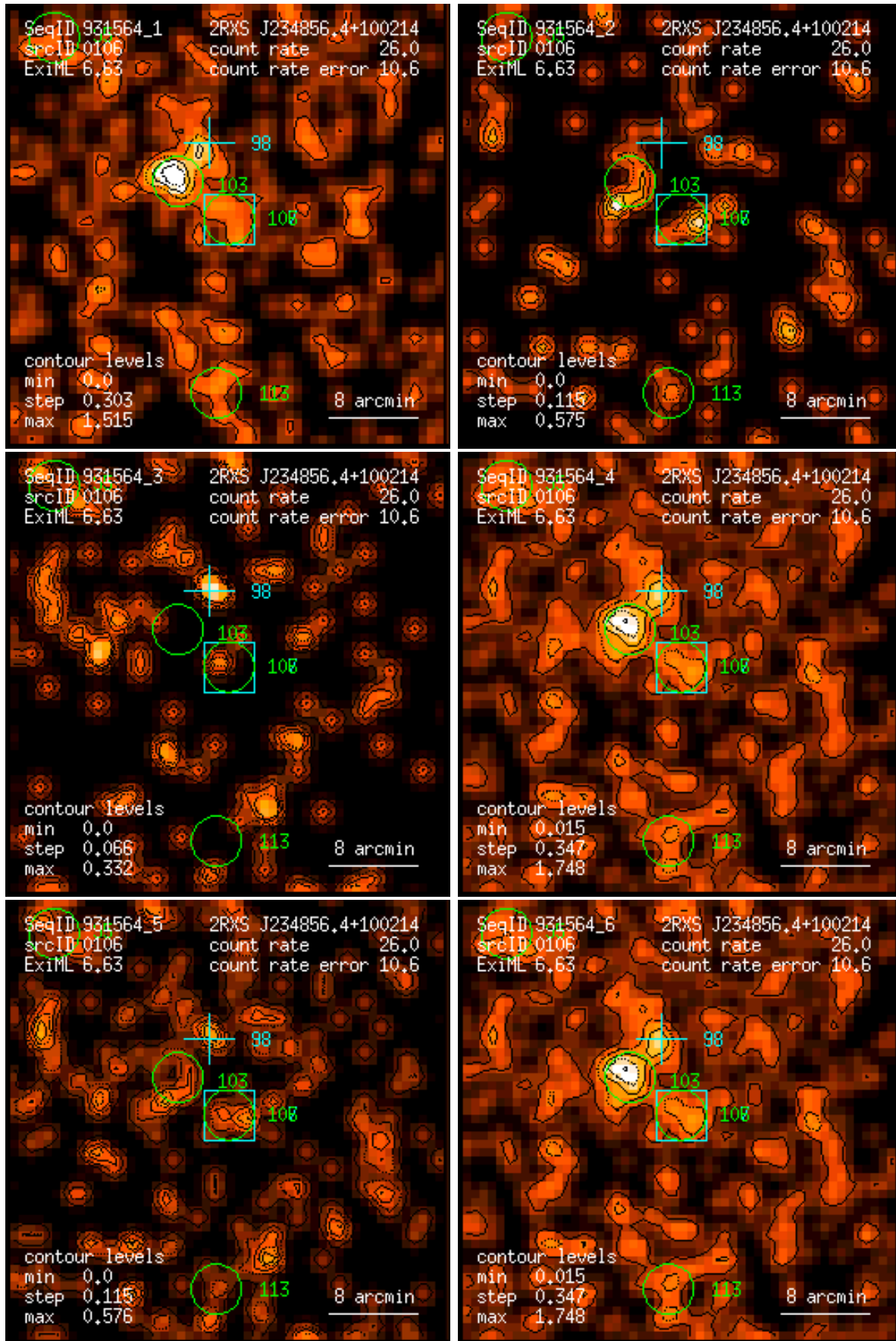
Figure 106: RASS 931564: detection 0106: band rate images, Gaussian filter: (1) PSPC channels 11 – 41, (2) 52 – 90, (3) 91 – 201, (4) 11 – 235, (5) 52 – 201, (6) 11 – 201. Broad band rates in counts/ks. Band rate contour levels in counts/ks/arcmin 2 .
