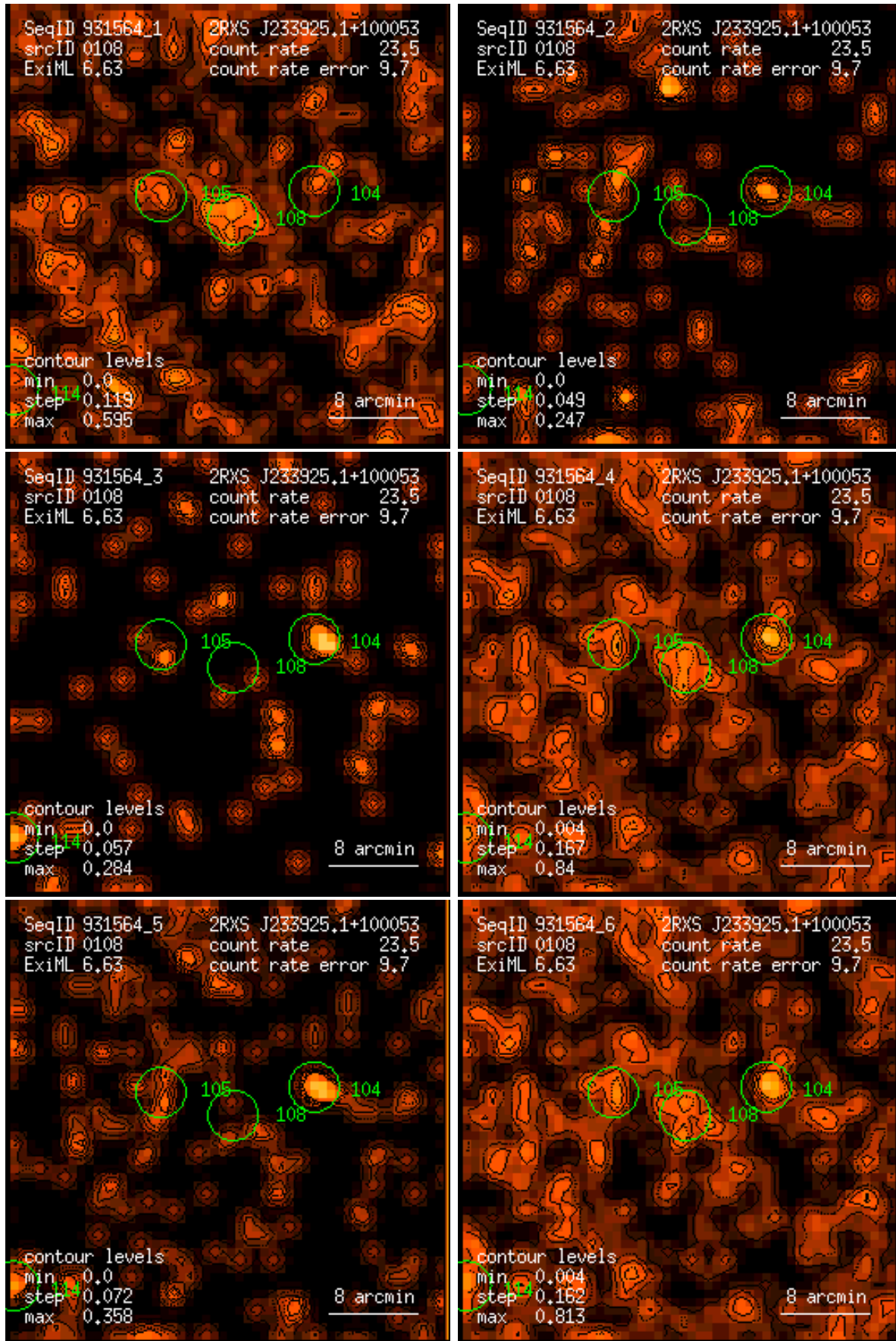
Figure 108: RASS 931564: detection 0108: band rate images, Gaussian filter: (1) PSPC channels 11 – 41, (2) 52 – 90, (3) 91 – 201, (4) 11 – 235, (5) 52 – 201, (6) 11 – 201. Broad band rates in counts/ks. Band rate contour levels in counts/ks/arcmin 2 .
