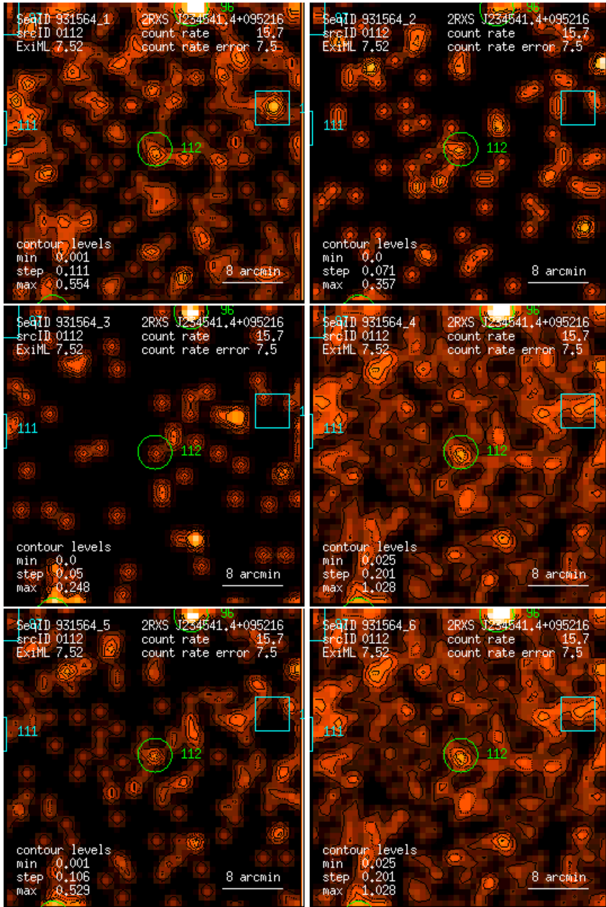
Figure 112: RASS 931564: detection 0112: band rate images, Gaussian filter: (1) PSPC channels 11 – 41, (2) 52 – 90, (3) 91 – 201, (4) 11 – 235, (5) 52 – 201, (6) 11 – 201. Broad band rates in counts/ks. Band rate contour levels in counts/ks/arcmin 2 .
