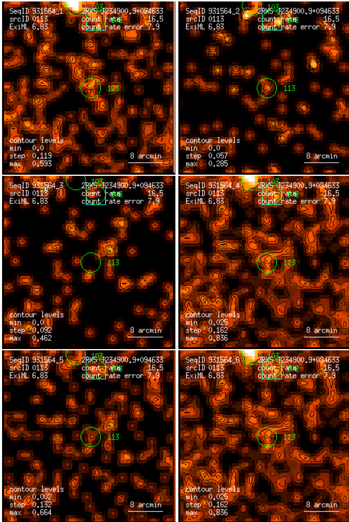
Figure 113: RASS 931564: detection 0113: band rate images, Gaussian filter: (1) PSPC channels 11 – 41, (2) 52 – 90, (3) 91 – 201, (4) 11 – 235, (5) 52 – 201, (6) 11 – 201. Broad band rates in counts/ks. Band rate contour levels in counts/ks/arcmin 2 .
